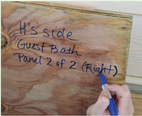
Figures 4-20 and 4-21. Not only is it necessary to install plywood opening covers correctly, it is also important to correctly label them and store them away from heat and humidity. Images courtesy of Dennis Hwang
