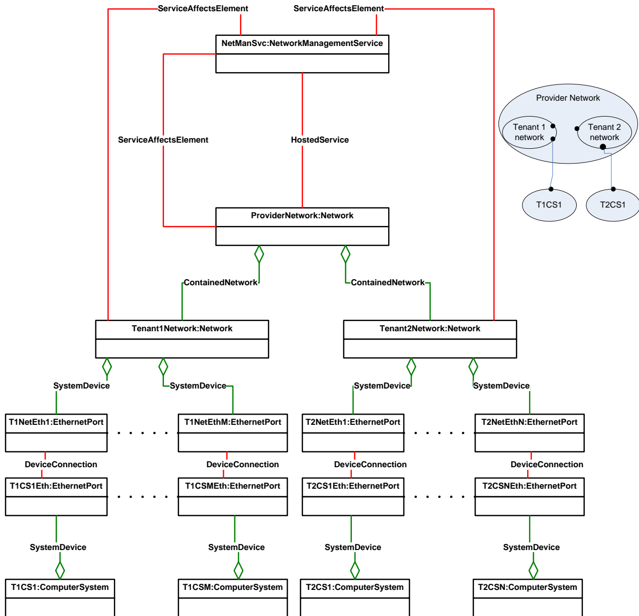
637 Figure 8 – Representing systems connected to ethernet ports of two tenant networks within a 638 provider network
