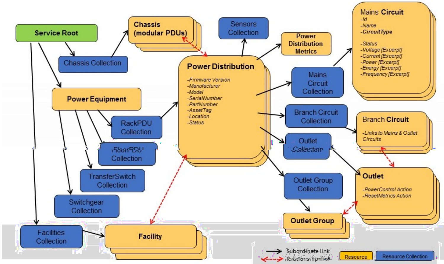
Figure 1: Resource Tree for a Power Distribution Unit
