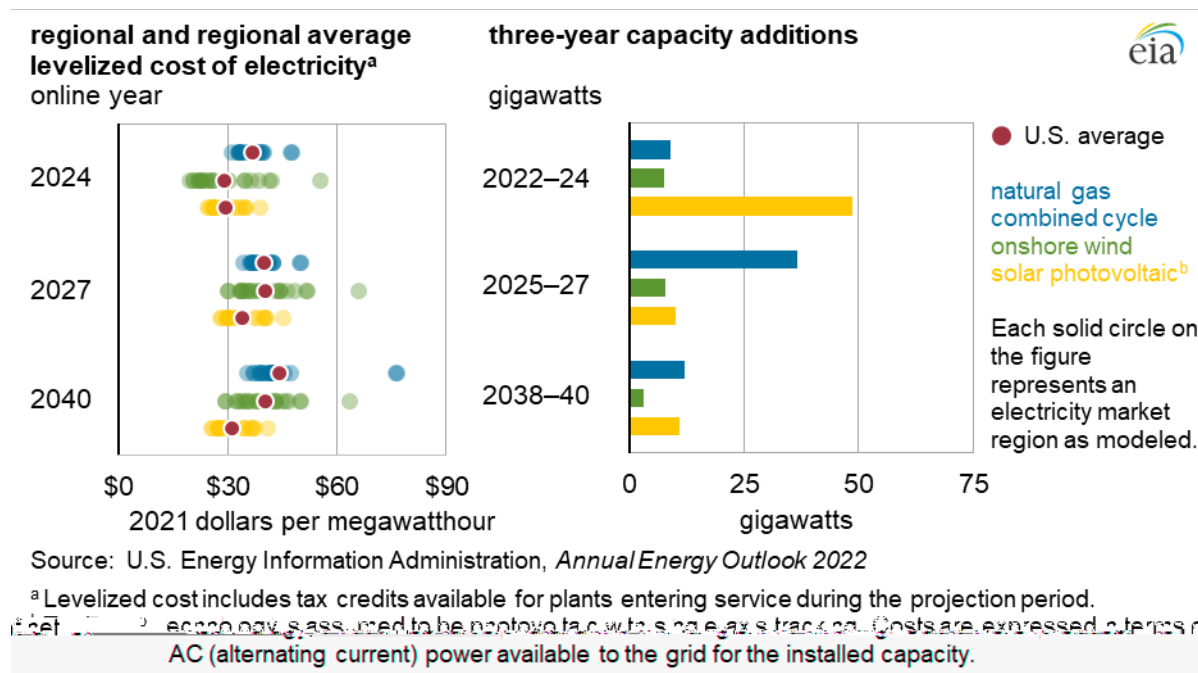
Figure 1. Levelized cost of electricity (with applicable tax subsidies) by region and total incremental capacity additions for selected generating technologies entering into service in 2024, 2027, and 2040
