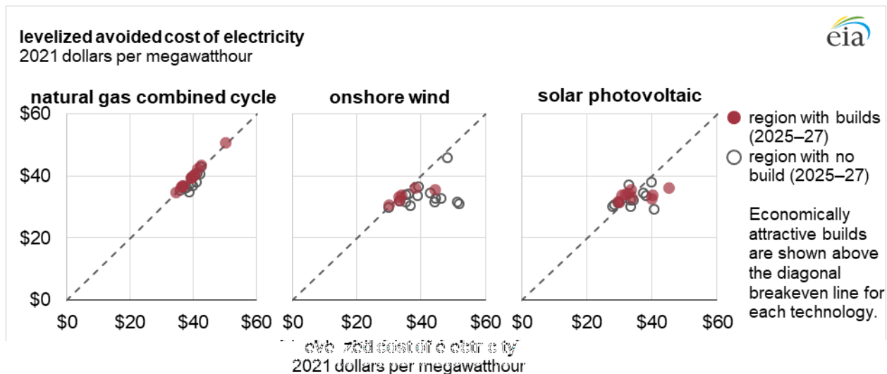
Figure 2. Levelized cost of electricity and levelized avoided cost of electricity by region for selected generation technologies, 2027 online year
