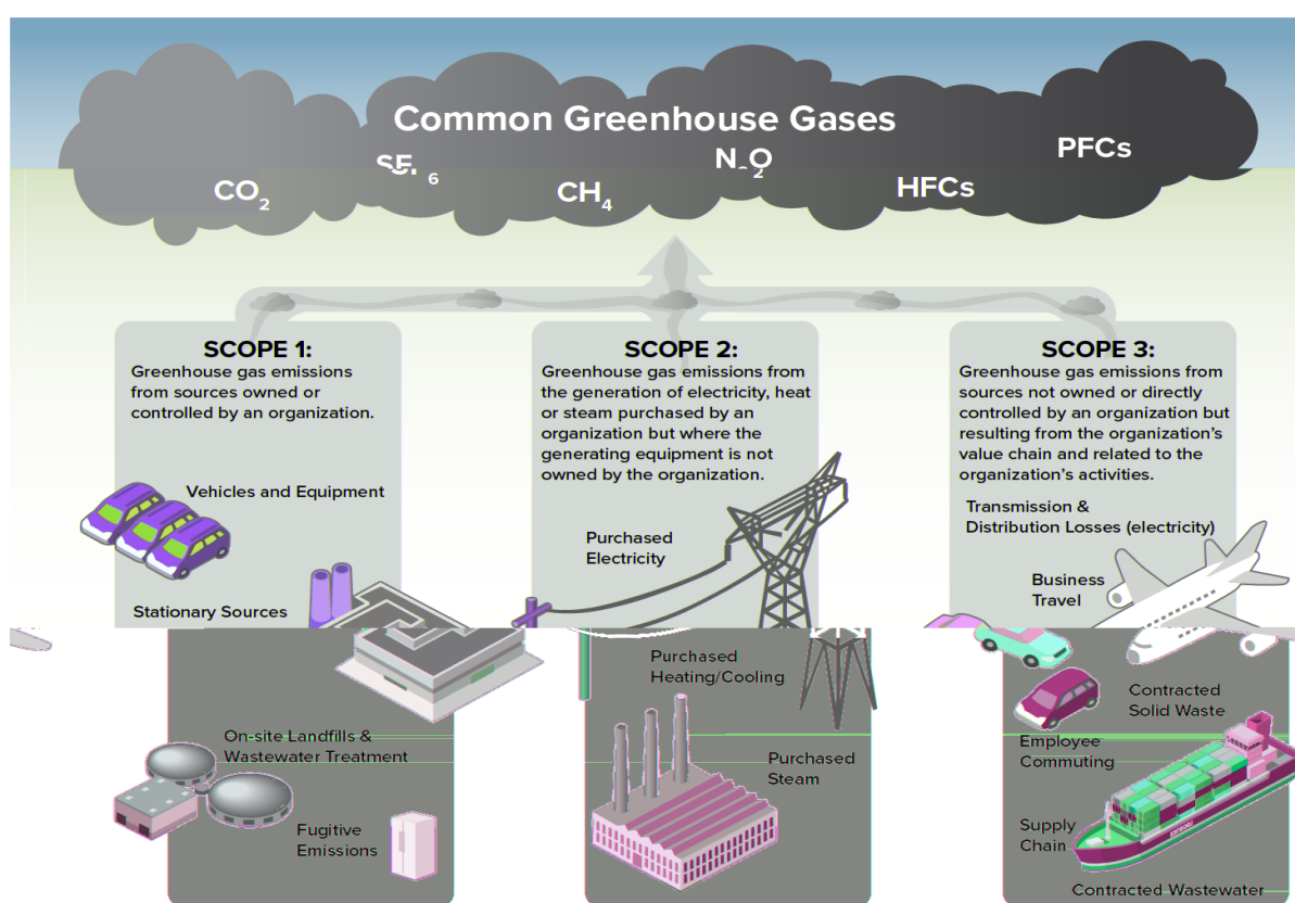
Figure 1. Common Sources of Emissions by Scope
