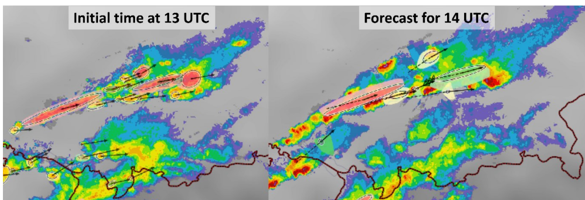
12 July 2023 observed radar reflectivity, ESWD reports in last 3 hours, and KONRAD3D-EPS pseudo member product shown for the nowcast initial time at 13 UTC and forecast for 14 UTC.
