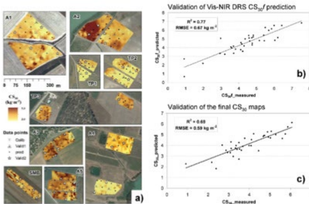
Fig. 1: Predicted maps of carbon stock CS_{30} with calibration and validation sites (a). On the right, the validation results of carbon stock of the fine earth (< 2mm, CS_{30}f ) predicted by Vis-NIR DRS (b) and the final validation of the maps after geographical weighted multiple regression, using \gamma -ray maps as covariates (c). The images and the results of this work was already published in Priori et al. 2016 .
