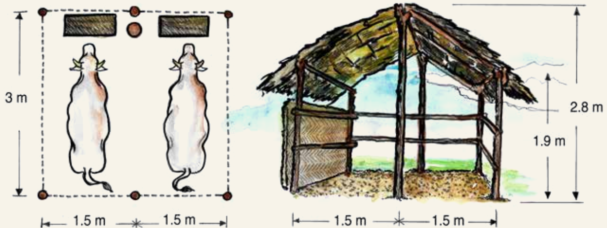
Plate 4.4 Simple shed for working cattle
