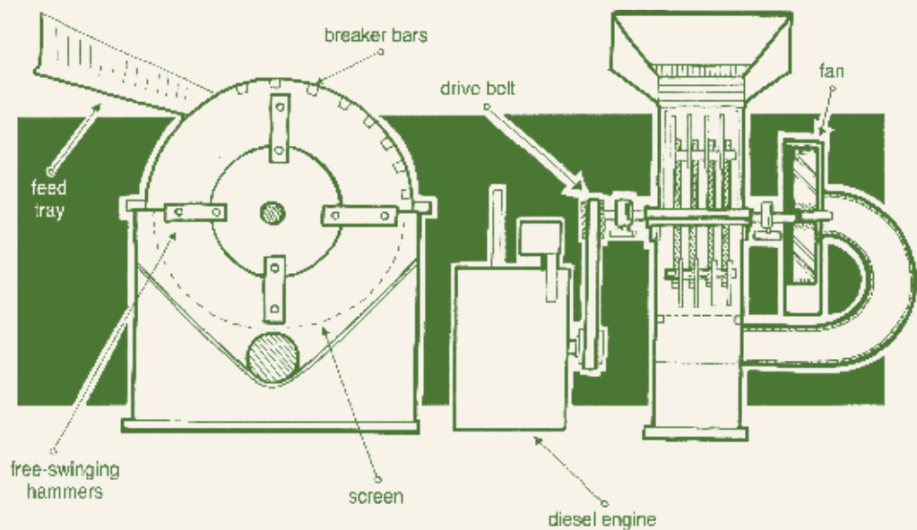
Plate 1.12 Hammer mill
