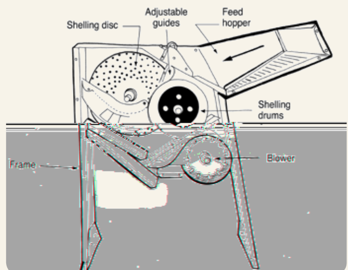
Plate 4.15 Maize sheller with blower
