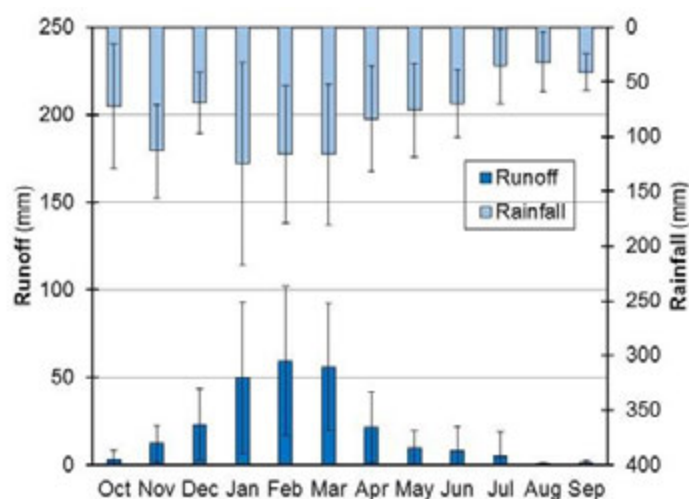
Figure 1: Monthly average rainfall and runoff at La Tejería watershed (2007-2016). Vertical bars are standard deviation. Similar pattern was observed in the remaining watersheds.
