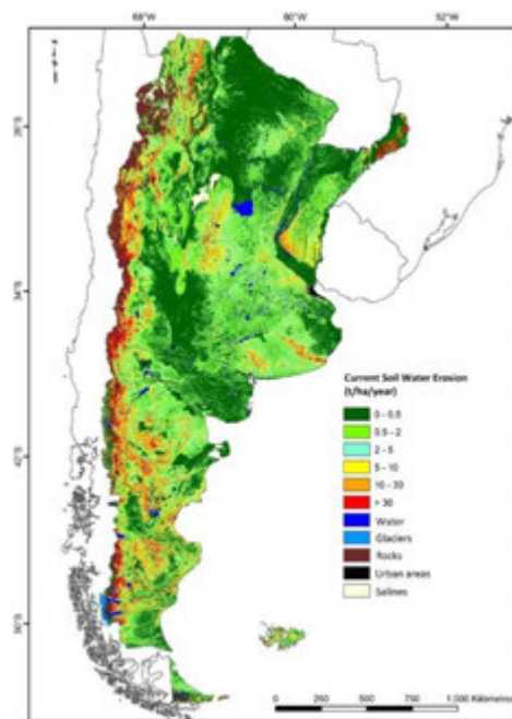
Figure 1: Current soil water erosion in Argentina.
