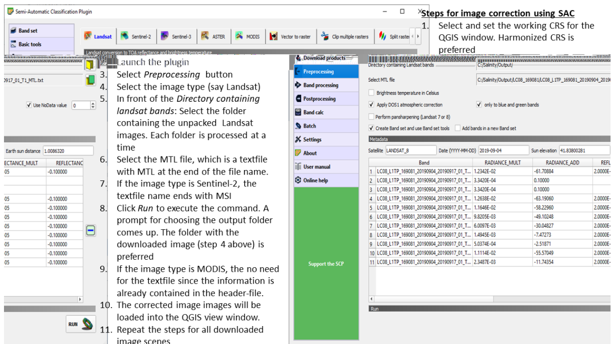
Figure 4.8: Image processing using semi-automatic classification plugin
