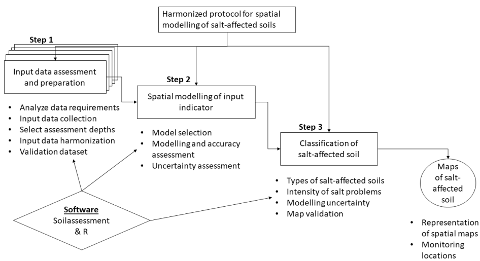
Figure 2.1: Approach for national mapping salt-affected soils
