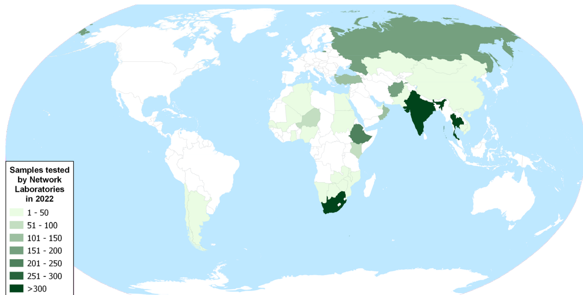
Figure 2: Samples received during 2022 from FMD outbreaks (routine surveillance that is undertaken in countries that are FMD-free without vaccination is not shown). Data from presentations given at the WOAHO/FAO FMD reference laboratory network annual meeting ( https://www.foot-and-mouth.org/Ref-Lab-Network/Network-Annual-Meeting ).
