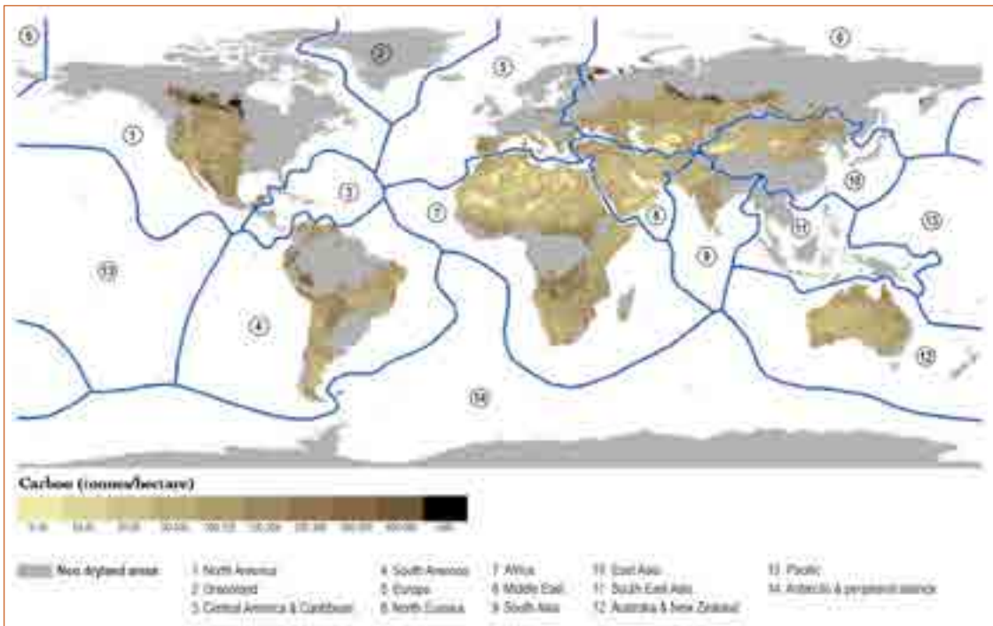
Figure 11 · Carbon mass per hectare throughout the drylands. From United Nations, 2011
