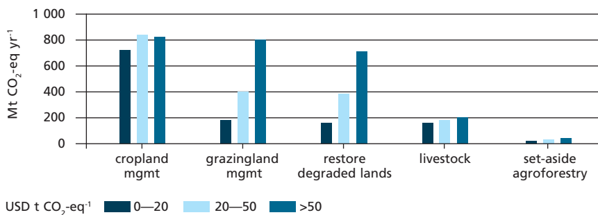
FIGURE 4: Estimates of carbon sequestration potential for several mitigation measures at varying carbon prices
