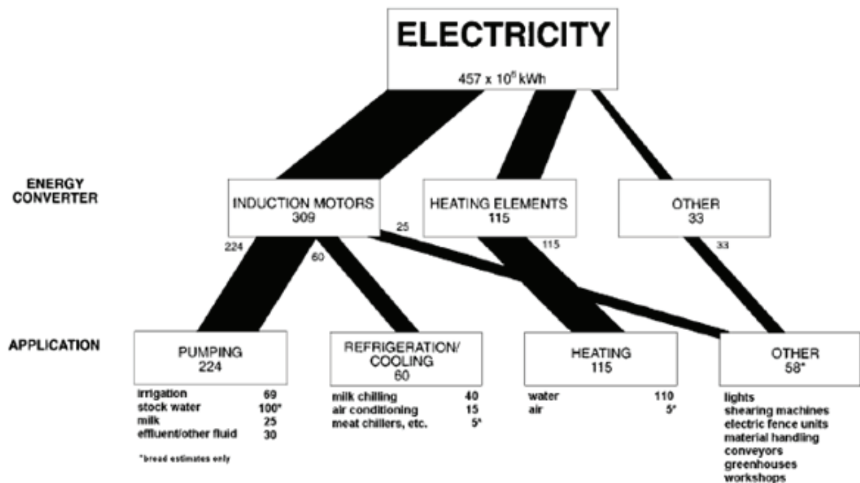
Figure A1. Energy flows of electricity demand on New Zealand farms in 1980 - an example of the detailed analysis of energy in the food sector conducted around that time. Source: NZERDC, 1983
