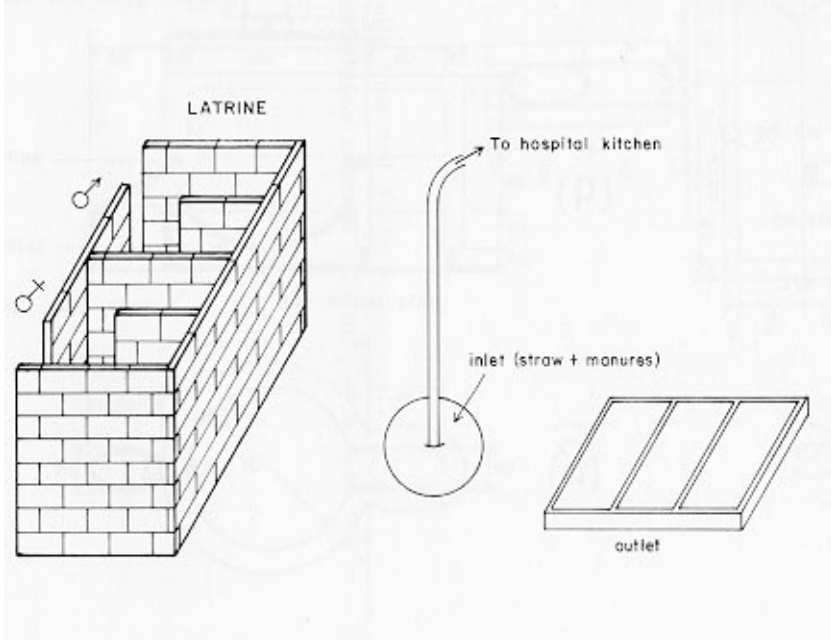
Fig. 41 43\text{ m}^3 BIOGAS UNIT FOR THE HOSPITAL OF TA HEH Commune (HEBEI Province)
