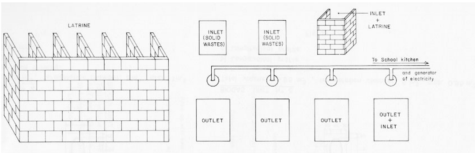
Fig. 40 13 BIOGAS UNITS 14\text{ m}^3 EACH, TA HEH MIDDLE SCHOOL, HUAI LU County, (HEBEI Province)
