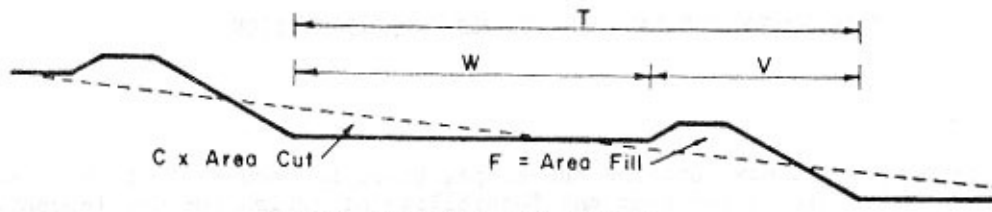
CROSS SECTION OF BENCH
