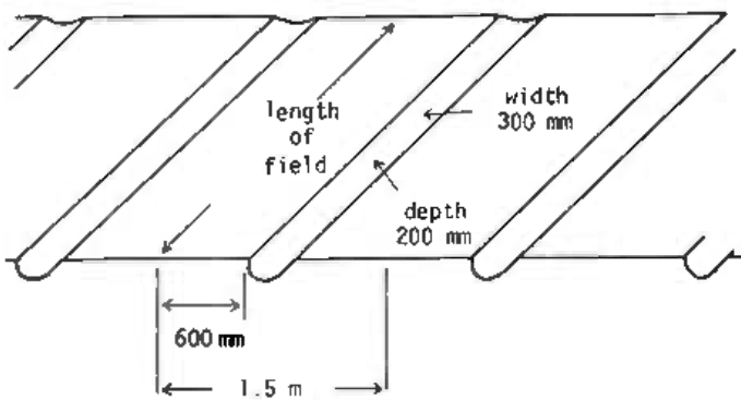
Figure 35 Broad based beds and furrows
