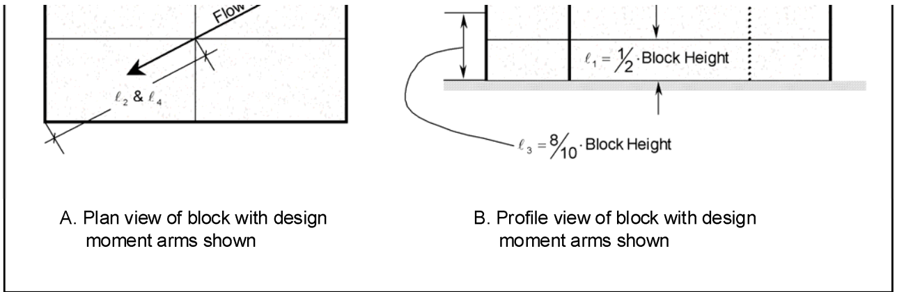
Figure 8.4. Schematic diagram of a block showing moment arms l_1 , l_2 , l_3 , and l_4 .
