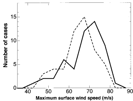
Fig. 2. Frequency distribution of maximum surface wind speeds obtained from the hurricane model in 51 case studies each from control (dashed line) and high-CO 2 (solid line) conditions.
