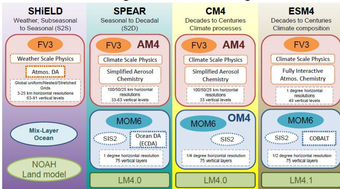
Figure 1: A schematic of GFDL model components and configurations.
