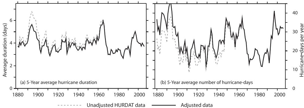
FIG. 2. Time series of 5-yr centered average (a) hurricane duration and (b) basinwide hurricane days per year based on the raw HURDAT data (dashed gray lines) and after adjusting presatellite records based on the estimated missed hurricanes (black lines). Units are (a) days per storm and (b) hurricane days per year.
