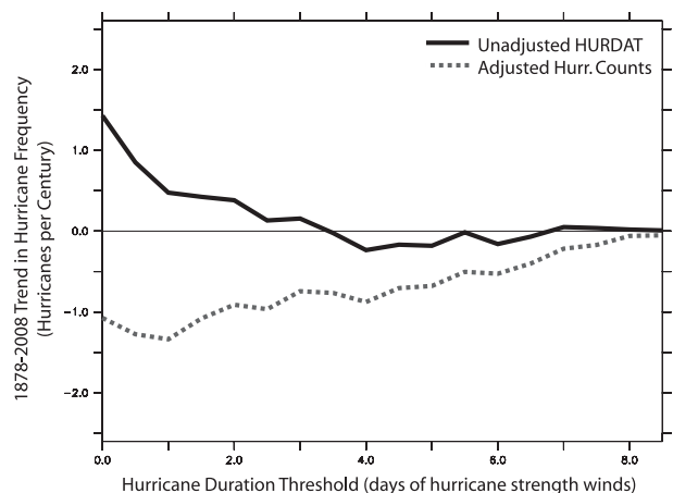
FIG. 3. Trends in North Atlantic basinwide hurricane frequency as a function of threshold duration of hurricane strength winds for raw HURDAT data (black line) and for the adjusted count data (gray dashed line). The threshold represents the number of days a storm had to have recorded winds \geq 33 \text{ m s}^{-1} ; the threshold is used for selecting the total number of storms in HURDAT for the entire record as well as the satellite-era storms that were used to compute the adjustment.
