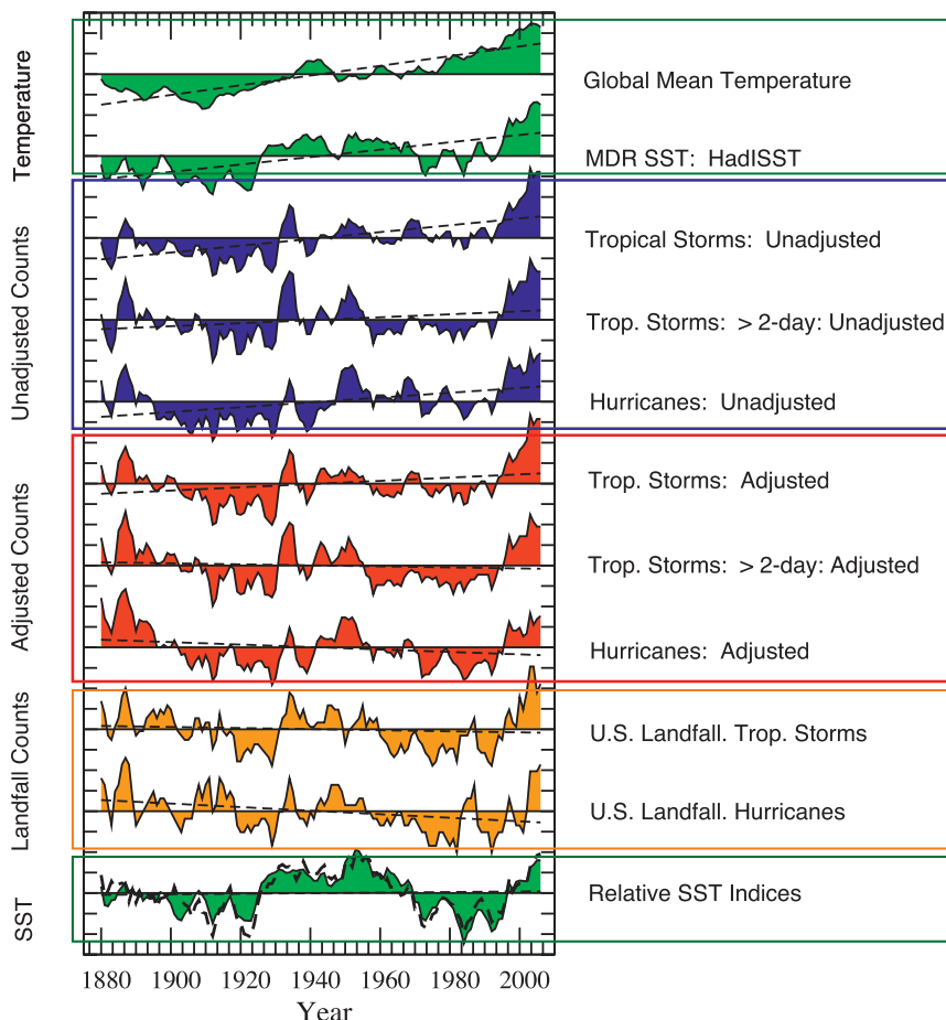
FIG. 5. Indices relevant to Atlantic tropical cyclone activity changes. Filled lines indicate the normalized 5-yr running means, during 1878–2008, with straight dashed lines indicating the linear least squares trends. Green-shaded curves depict global mean temperature [Hadley Centre Climatic Research Unit's land surface air temperature dataset, version 3 (HadCRUT3), August–October. MDR SST anomalies (HadISST; Rayner et al. 2003) and the relative SST (MDR minus tropical mean) from HadISST (Rayner et al. 2003) in solid; ERSSTv3b (Smith et al. 2008) in dashed. Blue-shaded curves represent unadjusted tropical storm and hurricane counts (HURDAT; Jarvinen et al. 1984; Landsea et al. 2008). Red curves include time-dependent adjustments for missing storms based on ship track density (VK08; Landsea et al. 2010) and for the adjusted hurricane count record from this study. Curves labeled >2-day depict storms with duration of at least 2 days (Landsea et al. 2010). Orange curves depict U.S. landfalling tropical storms and hurricanes (no adjustments). Vertical axis ticks represent one standard deviation, with all series normalized to unit standard deviation after a 5-yr running mean was applied. Only the top two temperature series—the unadjusted tropical storms of all duration and the unadjusted hurricane frequency series—have significant linear trends ( p = 0.05 ).
