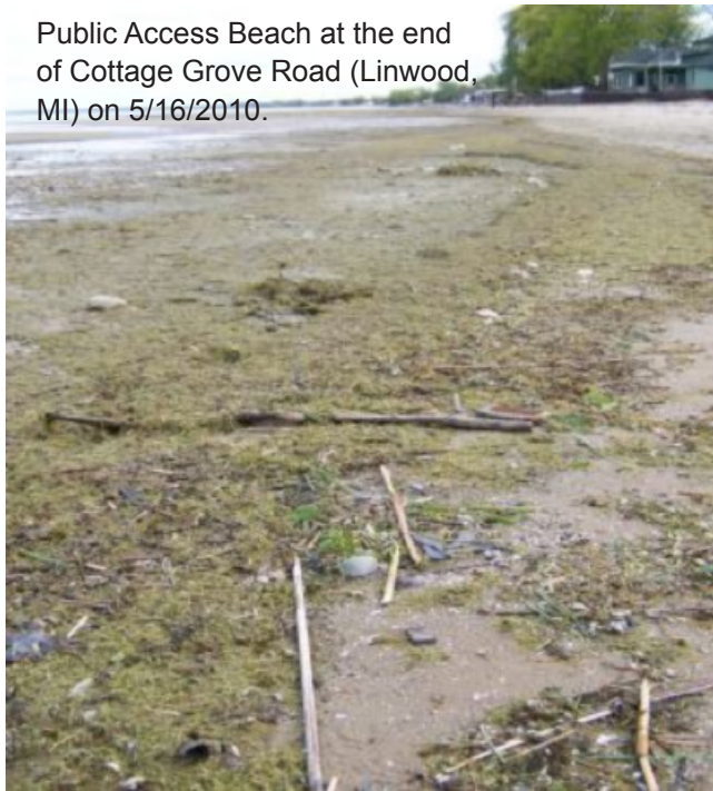
Figure 2.18 – Comparison of beach detritus between a location north of the Bay City Recreation Area (Linwood, MI) versus the wash-up at the Bay City Recreation Area (Bay City, MI) on the same day. Detritus at northern sites were less decomposed and more identifiable than material at the BCRA sites.
