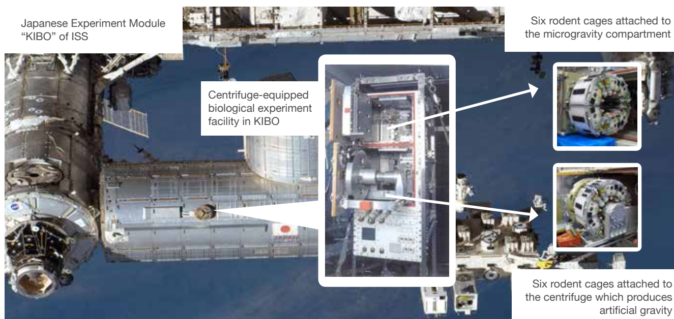
Figure 8: The Japan Aerospace Exploration Agency (JAXA) newly developed mouse habitat cage units that can be installed in the centrifuge-equipped biological experiment facility in the Japanese Experiment Module (“Kibo”) of ISS. The facility provides both microgravity (□g) and artificial gravity environments. Earth’s gravity (1 g), the Moon’s gravity (0.16 g) and Mars’ gravity (0.38 g) on the bottom floor of the cage can be mimicked by the rotating the centrifuge at 77, 31 and 48 rpm, respectively. In the first mission conducted in 2016, 12 mice were launched, divided into two groups of 6 mice each, and housed under □g or artificial earth-gravity (1 g). After 35 days of habitation in ISS, all mice were returned to the Earth in a live condition (image courtesy of JAXA).
