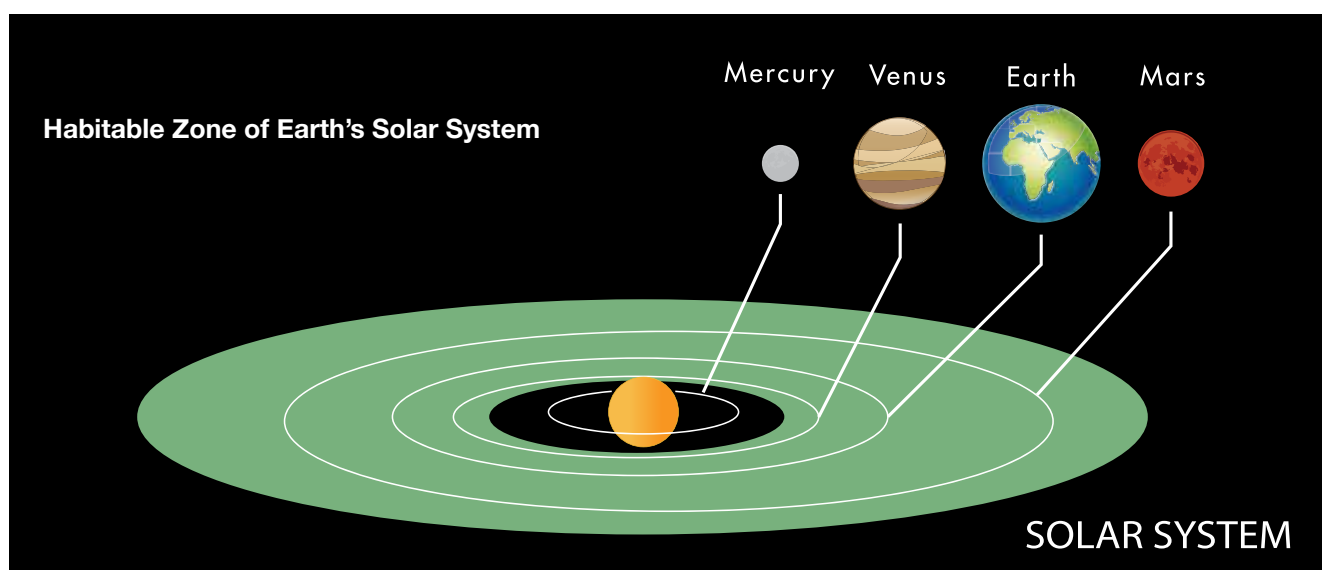
Figure 4: A key topic of the science that will be enabled by human exploration into the solar system is connected to the co-evolution of life with the planetary environment and life sciences. The current exploration destinations where humans can go are within the so-called habitable zone of Earth's solar system, i.e. the orbital distance from the Sun where the environmental conditions allow for liquid water to exist on the planetary surface. (Image courtesy of ESA)
