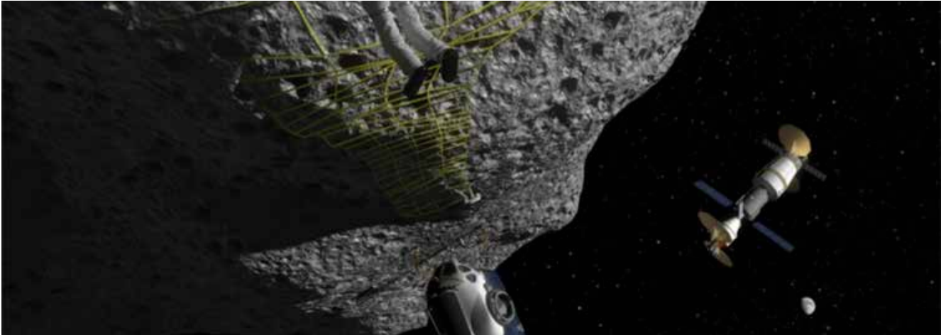
Figure 13: Astronauts visiting an asteroid would be able to handle delicate scientific instrumentation that could provide information on the internal structure of asteroids. This is of scientific interest, and it can also help with planetary defence.
