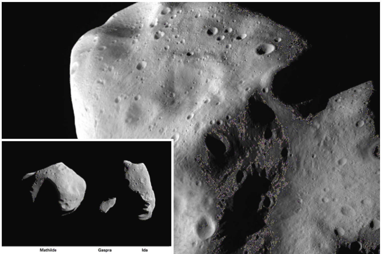
Figure 12: Asteroids are remnants of the early history of our Solar System and provide many scientific clues to its formation. The above images show different asteroids that were imaged by space probes in recent years. (Image courtesy of ESA)
