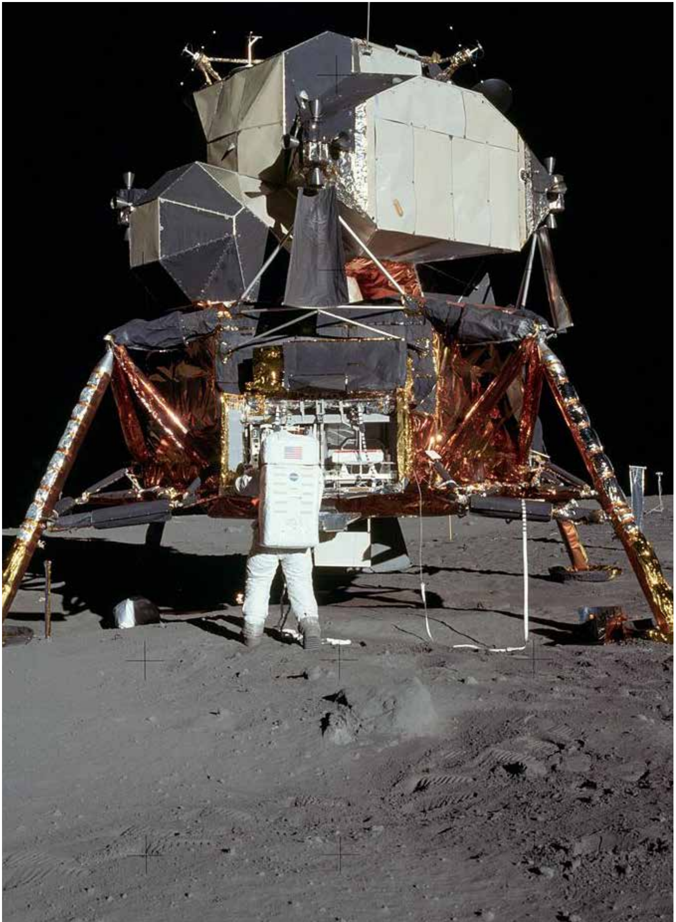
Figure 3: One particular value of humans for planetary surface science is the ability to emplace and to service delicate scientific instruments. The Apollo missions brought important science packages to the lunar surface that were deployed by the astronauts and continued to deliver high-value science well beyond the human surface mission. (Image courtesy of NASA)
