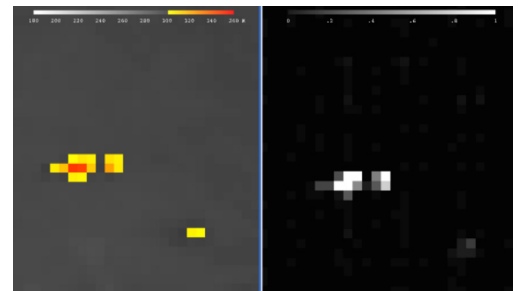
Nighttime AHI images over Australia on March 23, 2015 of bands 3.9 \mu\text{m} (left) and 1.6 \mu\text{m} (right) showing several fires. The AHI 1.6 \mu\text{m} band is nominally 2 km spatial resolution, while the ABI band will be 1 km. Credit: JMA/CIMSS
