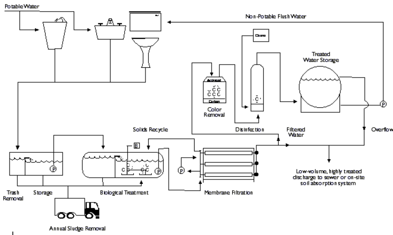
Figure 6-2. Combined Wastewater Treatment and Recycling System for a Commercial and Industrial Building.
