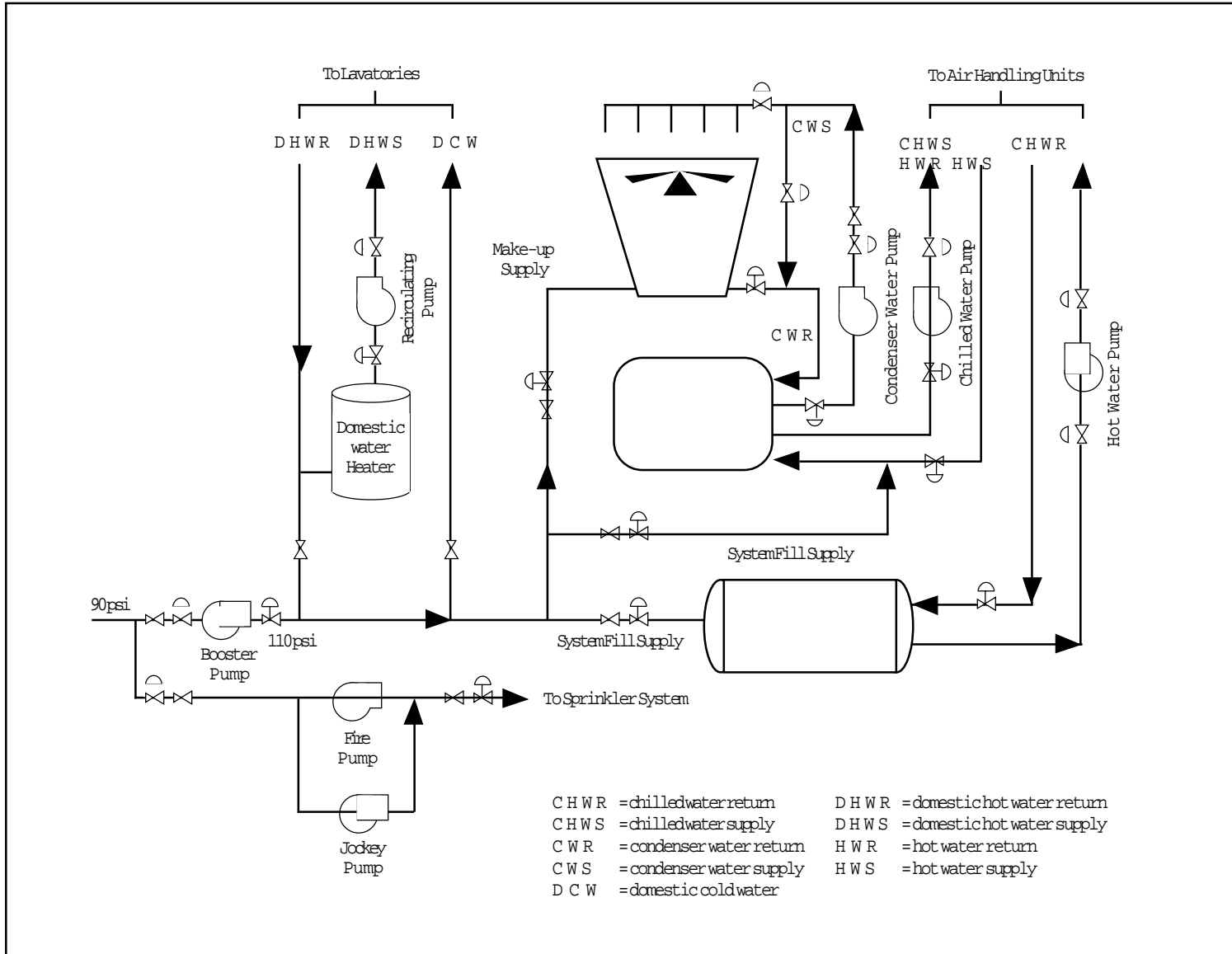
Figure 3-1. Water Balance Diagram.
