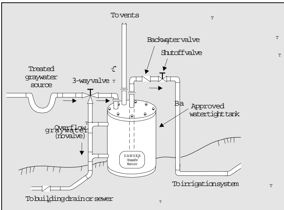
Figure 6-1. Typical Graywater Piping and Distribution System.
