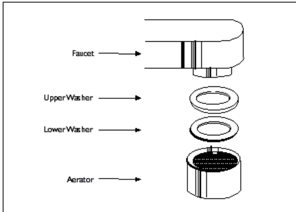
Figure 5-10. Faucet Aerator.
