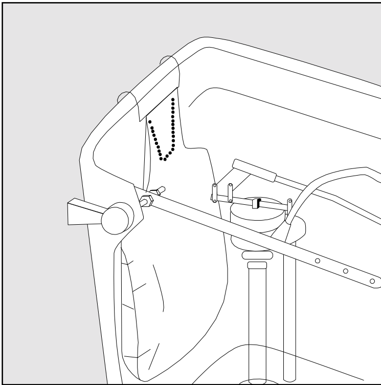
Figure 5-2. Toilet Displacement Bag.
