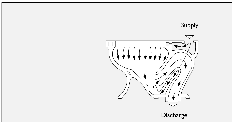
Figure 5-5. Blowout Toilet Schematic.
