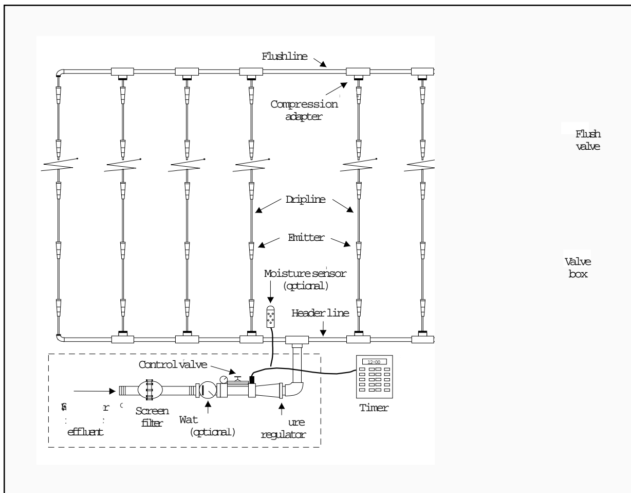
Figure 5-12. Subsurface Drip Irrigation System.
