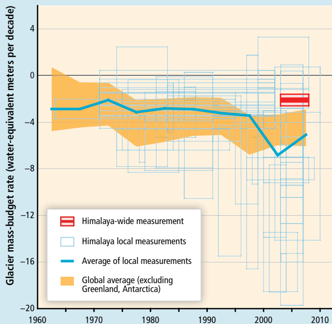
Figure 3-3 | All published glacier mass balance measurements from the Himalaya (based on Bolch et al., 2012). To emphasize the variability of the raw information, each measurement is shown as a box of height \pm 1 standard deviation centred on the average balance ( \pm 1 standard error for multiannual measurements). Region-wide measurement (Kääb et al., 2012) was by satellite laser altimetry. Global average (WGI AR5 Chapter 4) is shown as a 1-sigma confidence region.
