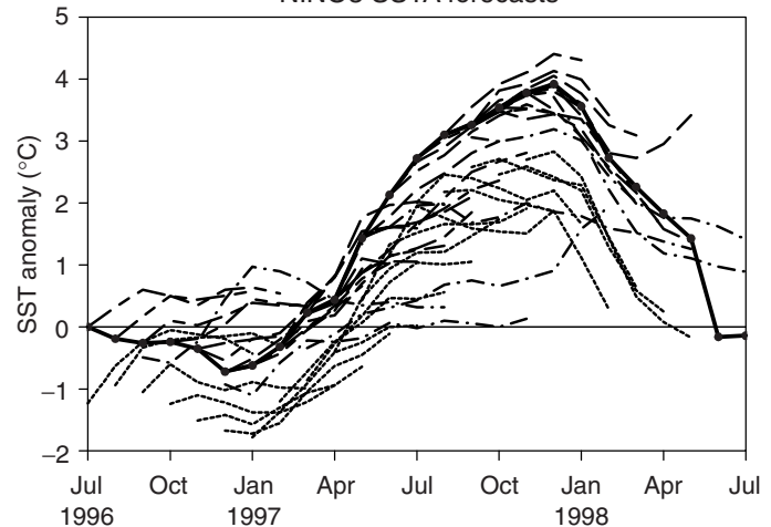
Figure 8.22: Niño-3 SSTA anomaly predictions and hindcast made at various times during the 1997 to 1998 El Niño event together with the subsequent observed SSTA anomaly (solid). Predictions made at ECMWF (Stockdale et al. , 1998, long dash), JMA (Ishii et al. , 1998, short dash), NCEP (Barnston et al. , 1999, long short dash) and the hindcast made at BMRC (Wang et al. , 2000, dot dash) are shown.
