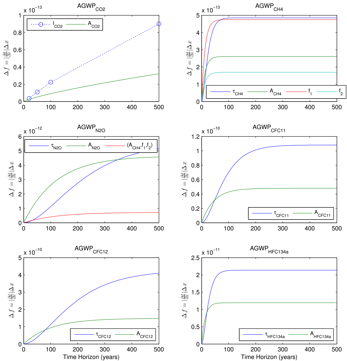
Figure 8.SM.6 | The contribution of each term to the uncertainty in the AGWP, \Delta AGWP is obtained by adding each term in quadrature according to Equation 8.SM.21. I_{CO_2} has data available only for four data points. For AGWP_{N_2O} the contribution from the radiative efficiency and indirect effect of CH 4 are combined in quadrature. In uncertainty analysis, the contributions are added in quadrature (Equation 8.SM.21), which will amplify the differences.
