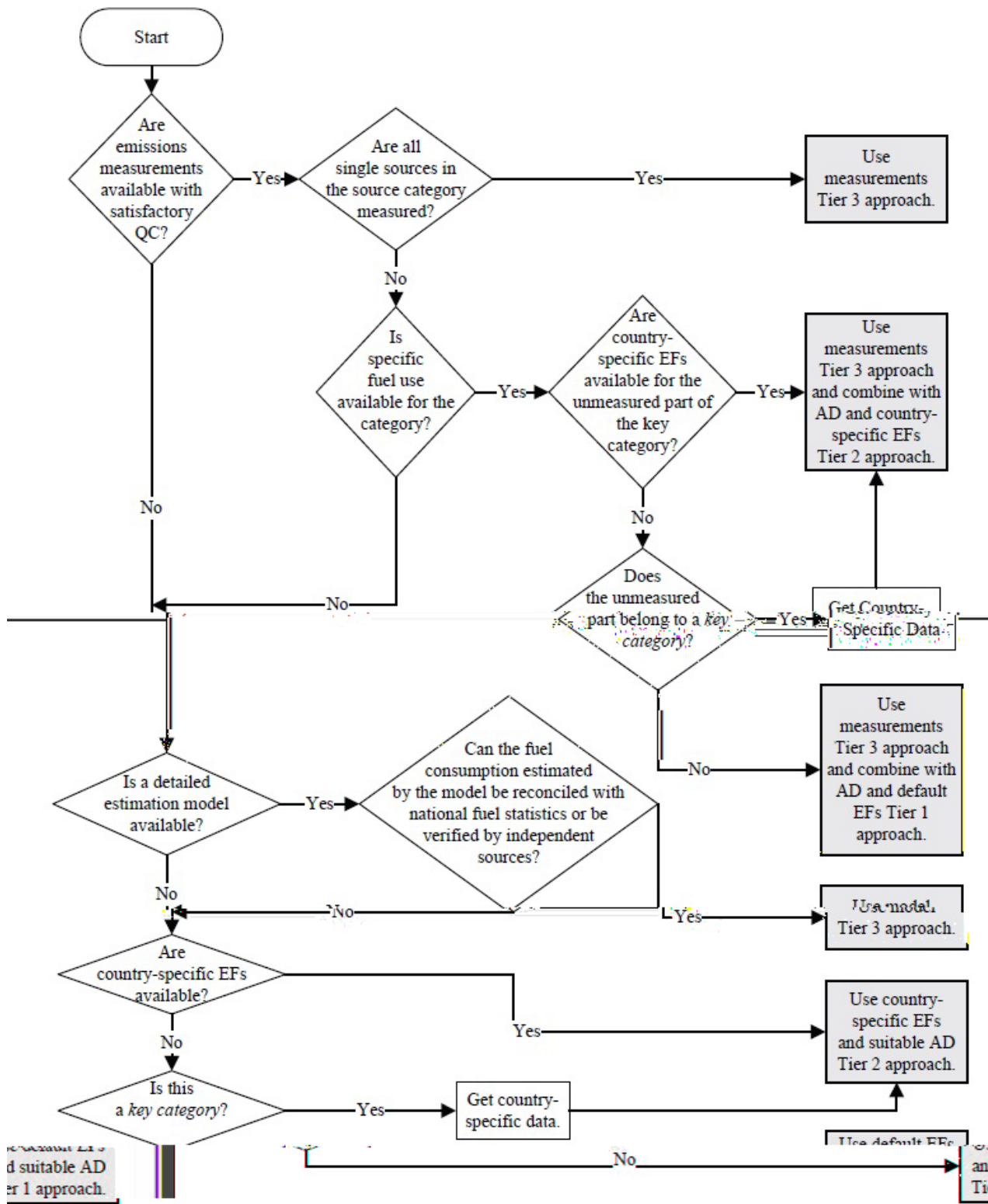
Figure 1.2 Generalised decision tree for estimating emissions from fuel combustion
