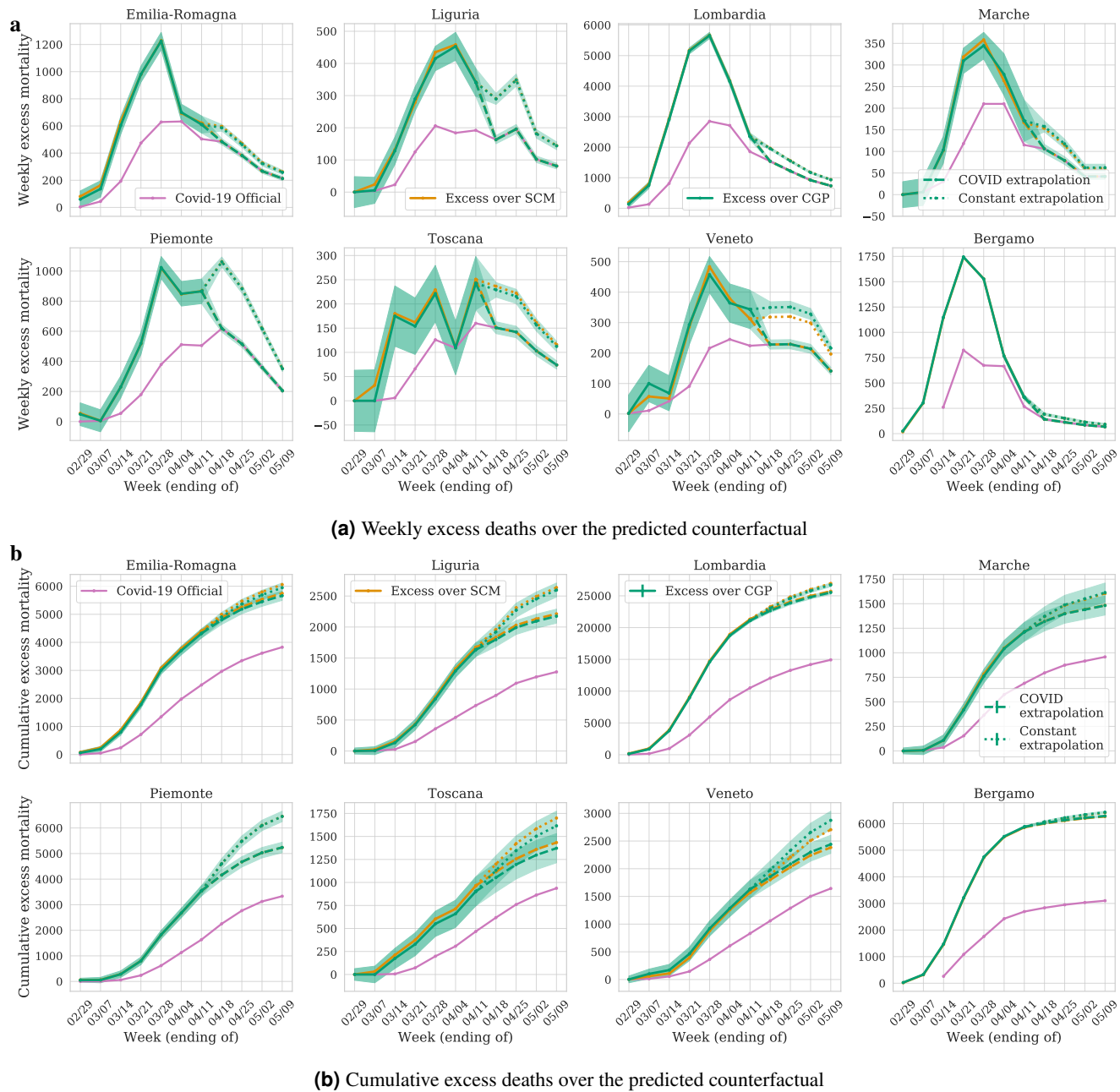
Figure 2. Excess mortality compared to reported COVID-19 deaths in regions of Northern Italy and the province of Bergamo. a , excess weekly deaths, and b , cumulative excess deaths, over the predicted counterfactual in comparison to the reported COVID-19 deaths (in pink) for the period since February 23rd (available COVID-19 data). Estimates from both the counterfactuals, SCM (orange) and CGP (green) agree. We find that COVID-19 deaths are under-reported by multiple factors for every period and every region. We extrapolate the data excess beyond April 11th with dashed-lines. To do this, we make the conservative assumption that the ratio of excess deaths to COVID-19 reported deaths is 1 after April 18th.
