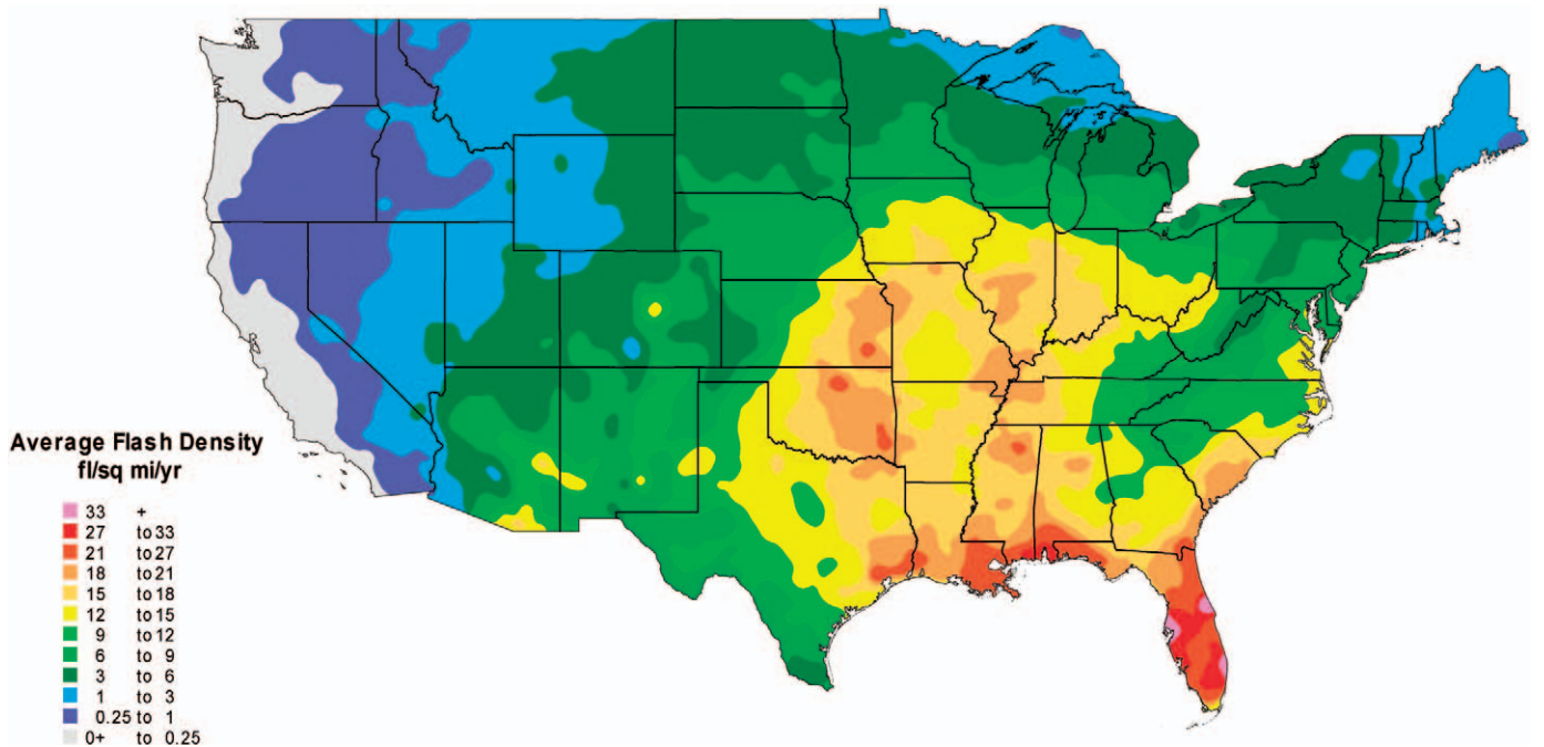
Figure 1. Lightning flash density, 2007–2011. National Lightning Detection Network. This map portrays the regions of highest cloud-to-ground lightning strikes (Florida and the Southeast) and the areas with the least frequent strikes (the West Coast and Western states). © Vaisala 2012. Reprinted with permission.
