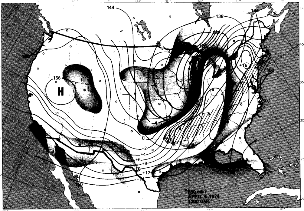
Figure 54 850-mb analysis, 1200 GMT, April 4, 1974. Contours, 60-m intervals; Isotherms, 2°C intervals; Dew point depressions \geq 20^{\circ}\text{C} , orange shading; Dew point depressions \leq 5^{\circ}\text{C} , gray shading; Wind speeds \geq 5 kn, hatched.
