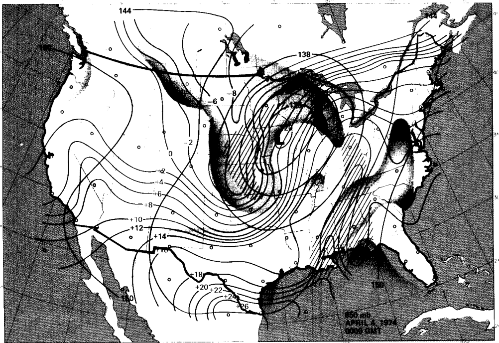
Figure 44 850-mb analysis, 0000 GMT, April 4, 1974. Contours, 60-m intervals; Isotherms, 2°C intervals; Dew point depressions \geq 20^\circ\text{C} , orange shading; Dew point depressions \leq 5^\circ\text{C} , gray shading; Wind speeds \geq 50 kn, hatched.
