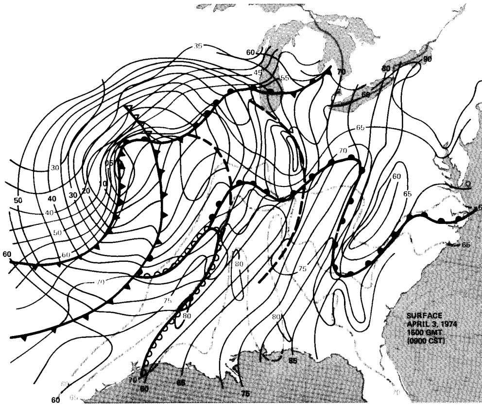
Figure 28 Surface analysis, 1500 GMT, April 3, 1974 (see legend in fig. 26).
