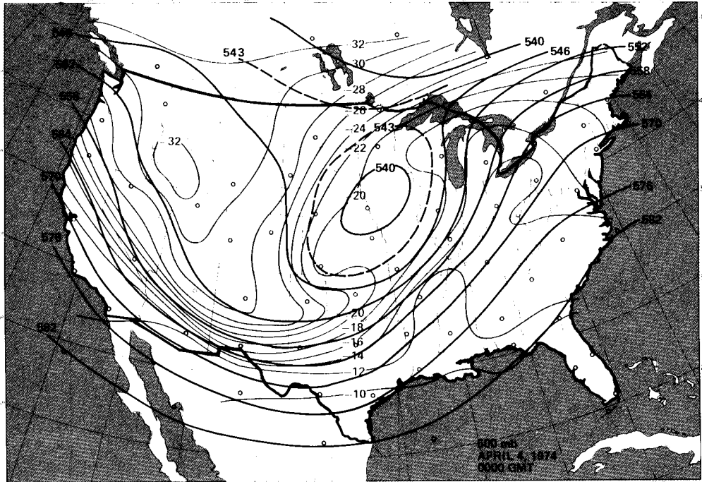
Figure 42 500-mb analysis, 0000 GMT, April 4, 1974. Contours, 60-m intervals; Isotherms, 2°C intervals.
