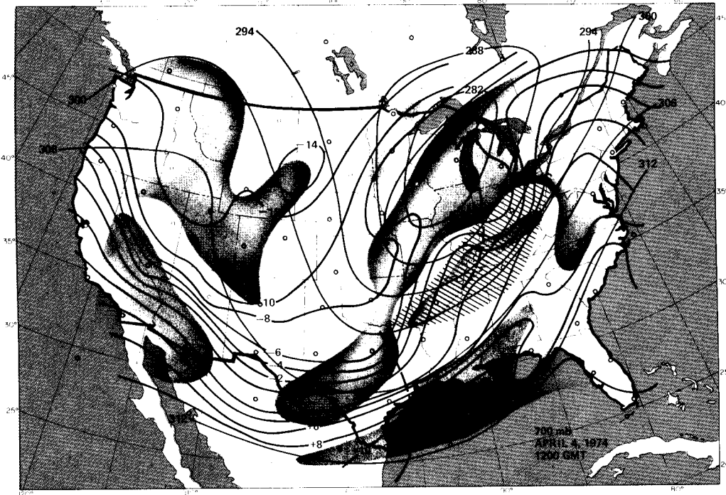
Figure 53 700-mb analysis, 1200 GMT, April 4, 1974. Contours, 60-m intervals; Isotherms, 2°C intervals; Dew point depressions \geq 20^{\circ}\text{C} , orange shading; Dew point depressions \leq 5^{\circ}\text{C} , gray shading; Wind speeds \geq 60 kn, hatched.
