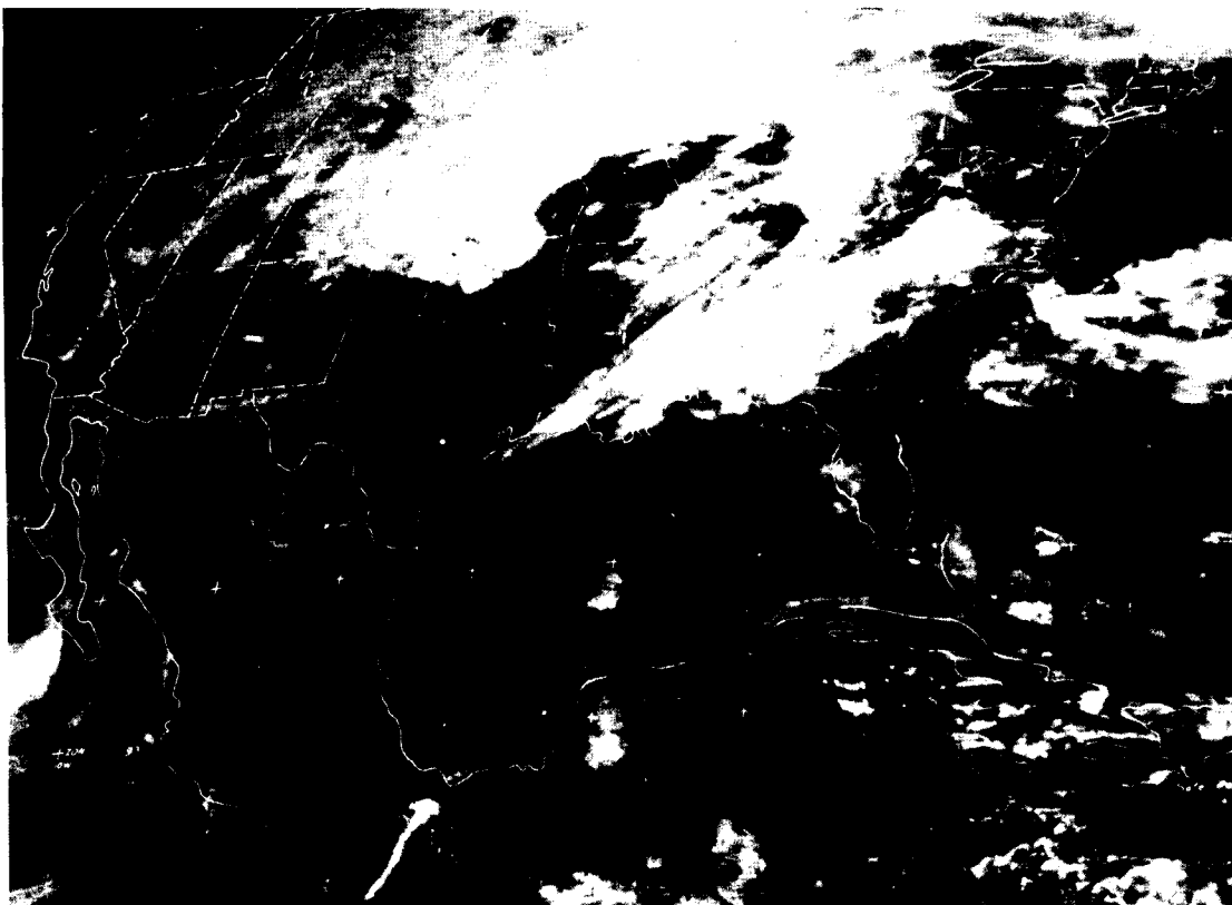
Figure 30 AT5-III photo, 1511 GMT, April 3, 1974.
