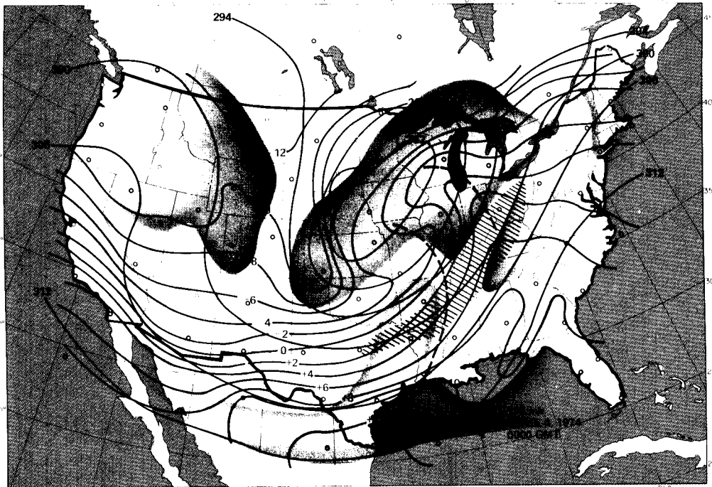
Figure 43 700-mb analysis, 0000 GMT, April 4, 1974. Contours, 60-m intervals; Isotherms, 2°C intervals; Dew point depressions \geq 20^\circ\text{C} , orange shading; Dew point depressions \leq 5^\circ\text{C} , gray shading; Wind speeds \geq 60 kn, hatched.
