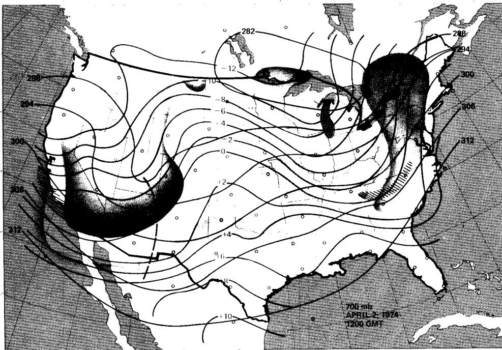
Figure 4 700-mb analysis, 1200 GMT, April 2, 1974. Contours, 60-m intervals; Isotherms, 2°C intervals; Dew point depressions \geq 20^\circ\text{C} , orange shading; Dew point depressions \leq 5^\circ\text{C} , gray shading; Wind speeds \geq 60 kn, hatched.
