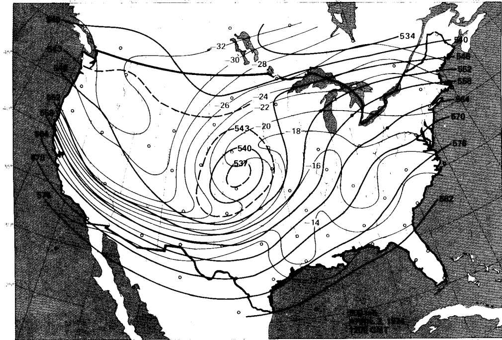
Figure 15. 500-mb analysis, 1200 GMT, April 3, 1974. Contours, 60-mb intervals; Isotherms, 2°C intervals.
