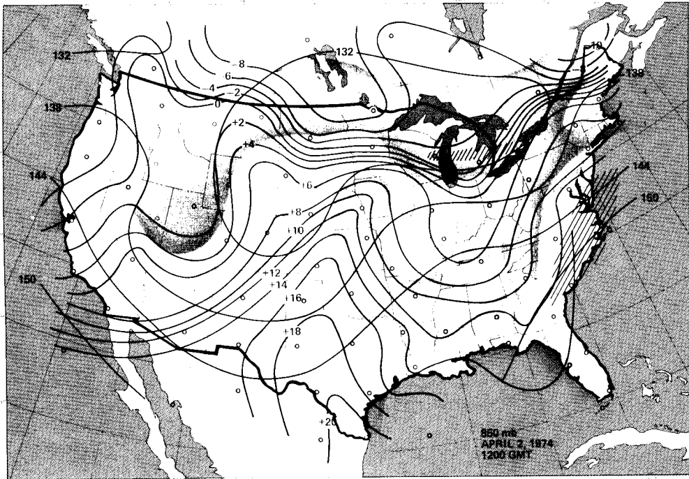
Figure 5 850-mb analysis, 1200 GMT, April 2, 1974. Contours, 60-m intervals; Dew point depressions \geq 20^\circ\text{C} , orange shading; Dew point depressions \leq 5^\circ\text{C} , gray shading; Wind speeds \geq 50 kn, hatched.
