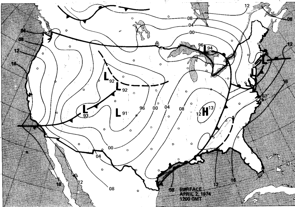
Figure 6 Surface analysis, 1200 GMT, April 2, 1974. Pressures, 4-mb intervals; 60^\circ\text{F} isodrosotherm, dashed.
