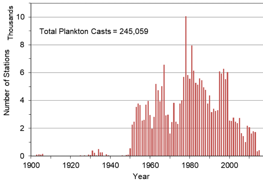
Figure 16.4. Temporal distributions of plankton casts in WOD23 as a function of year.
