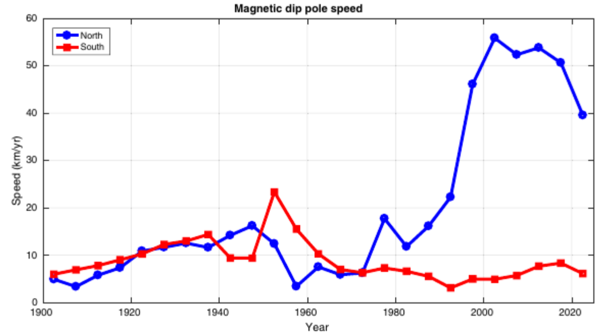
Fig. 4 Average speed of the magnetic dip poles over each 5-year epoch, plotted at the midpoint between epochs (i.e., the speed over 2015–2020 is shown at 2017.5). The value for 2020–2025 is a forecast
