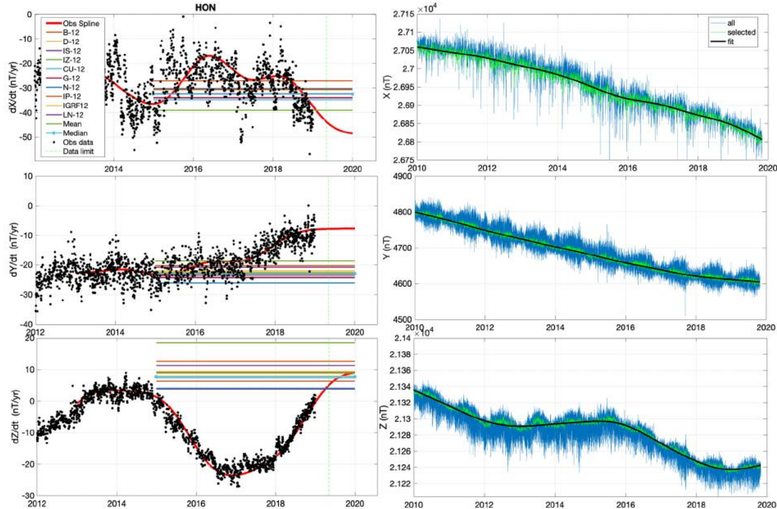
Fig. 12 IGRF12 retroactive SV comparison at Honolulu (HON). Left panels show the observatory annual differences of daily mean values (black), annual spline difference curve (red) and IGRF12 candidate predictions for the dB_x/dt (top), dB_y/dt (middle), and dB_z/dt (bottom) components in the NEC frame. Right panels show the original observatory data (blue), data after selecting for geomagnetically quiet periods (green), and fitted spline curve (black) for the B_x (top), B_y (middle) and B_z (bottom) components
