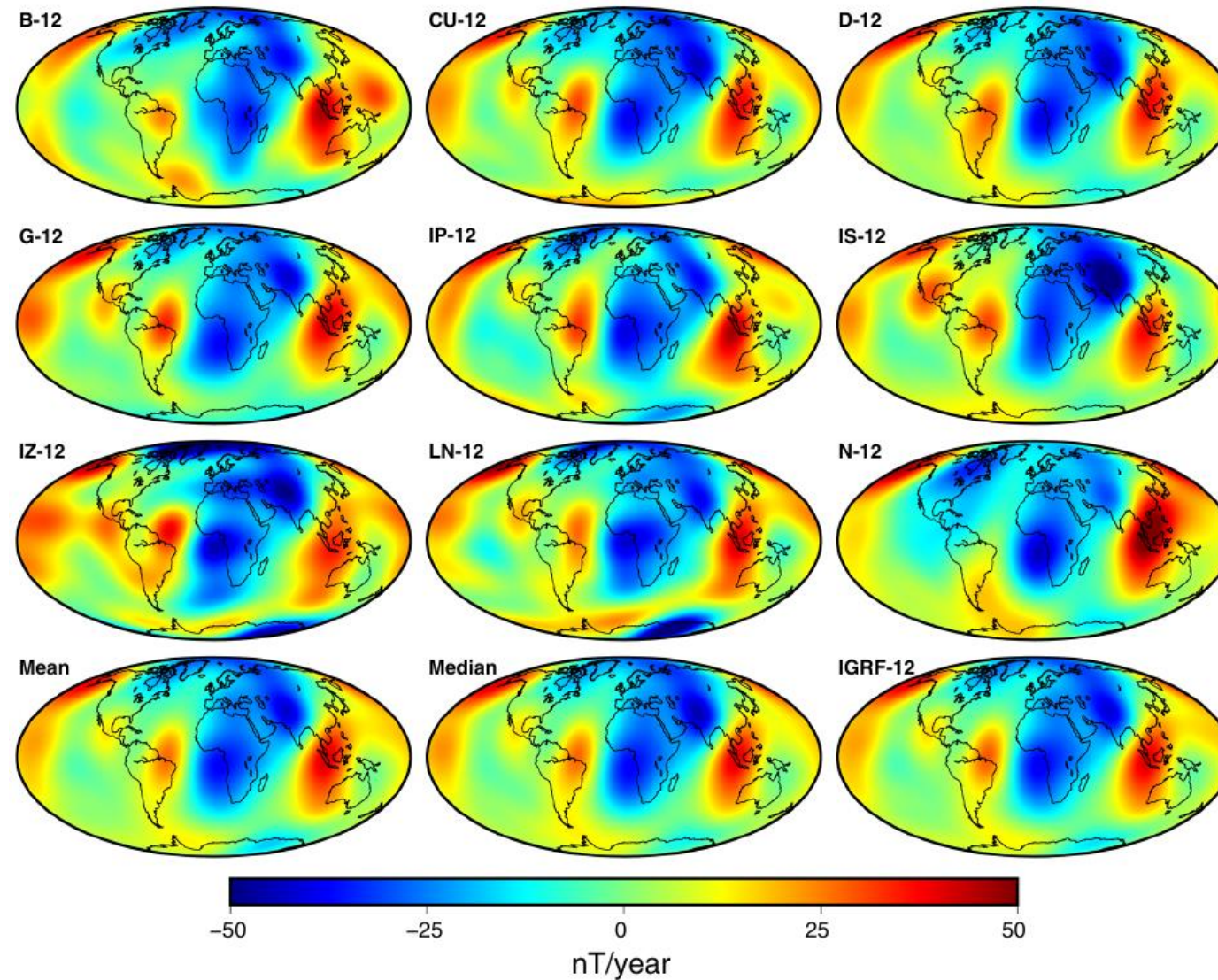
Fig. 13 Spatial map differences of dB_z/dt (in nT/year) between IGRF-12 secular variation candidates and final IGRF-13 secular variation model over the 2015.0 to 2020.0 time period. We additionally include spatial map differences (against IGRF-13) of the mean and median of all IGRF-12 candidates, as well as the final IGRF-12 SV model in the bottom row
