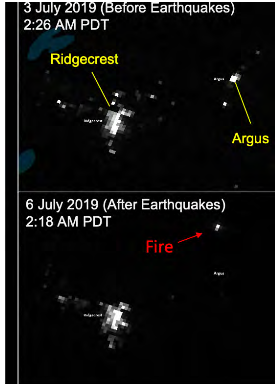
The 2019 Ridgecrest Earthquake intensity map (left), with DNB imagery showing both power outages around Ridgecrest and Argus (completely out), and a 'new light' from a fire.
