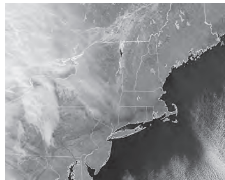
VIIRS high-resolution visible channel, I-1 (0.64 Qm), from NOAA-20 (17:09 UTC, 22 January 2019).
