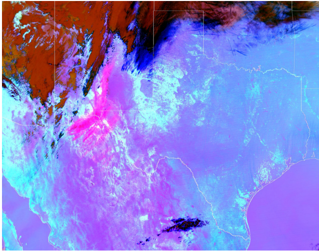
The VIIRS sensor aboard the JPSS Suomi-NPP captured a large dust storm (pink color) on March 31, 2017 over the northern Chihuahuah Desert (source: Shobha Kondragunta, NOAA).
