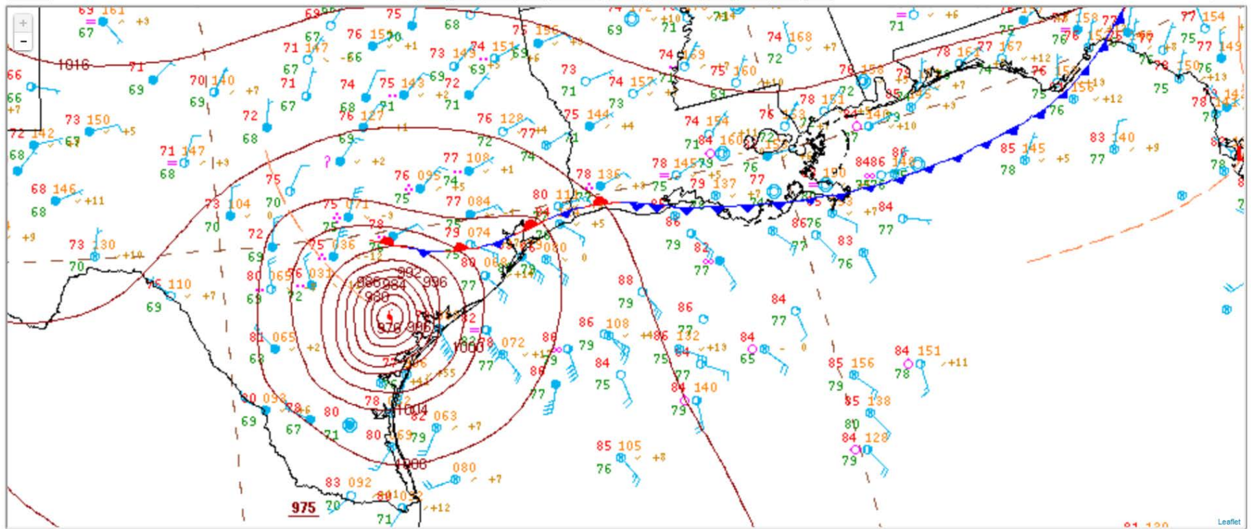
Figure 13. NCEP unified surface analysis at 1200 UTC 26 August 2017.
