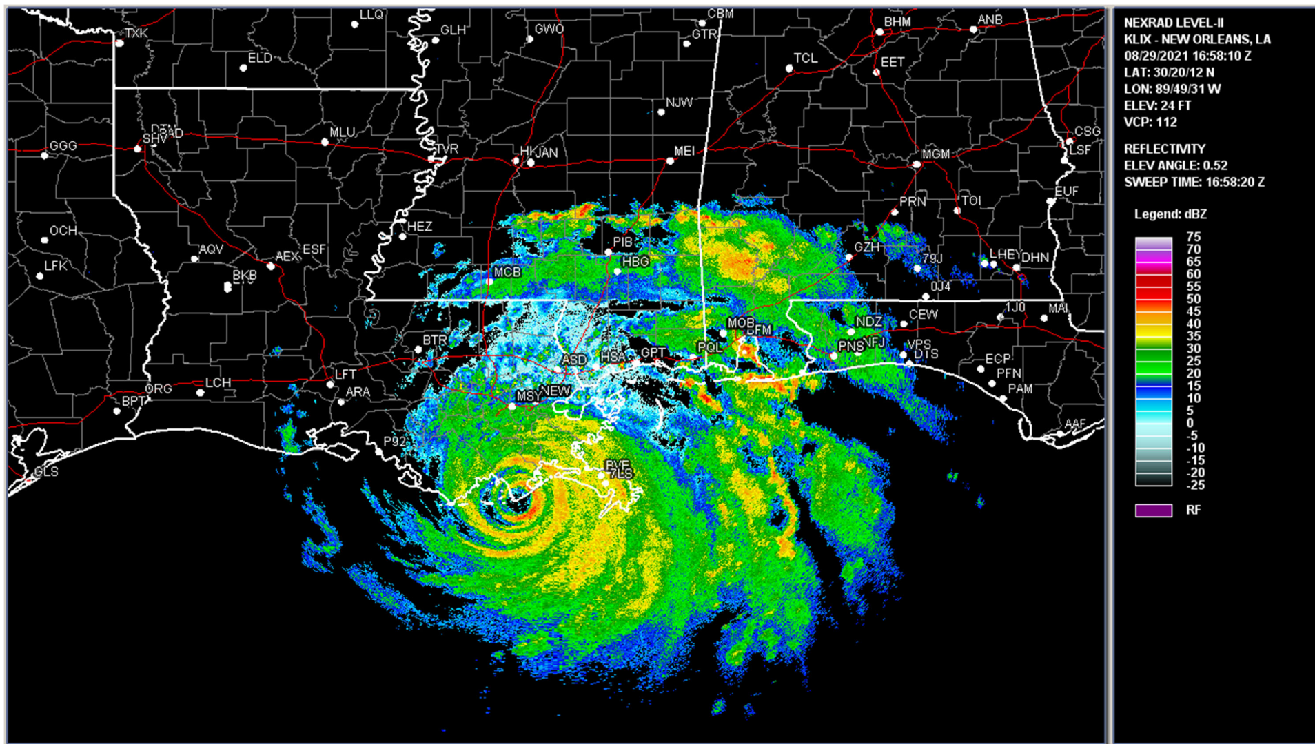
Figure 5. NWS Slidell WSR-88D radar reflectivity image of the eye of Ida making landfall at Port Fourchon, Louisiana, at 1658 UTC 29 August 2021. Image courtesy of NWS WFO Lake Charles, Louisiana.
