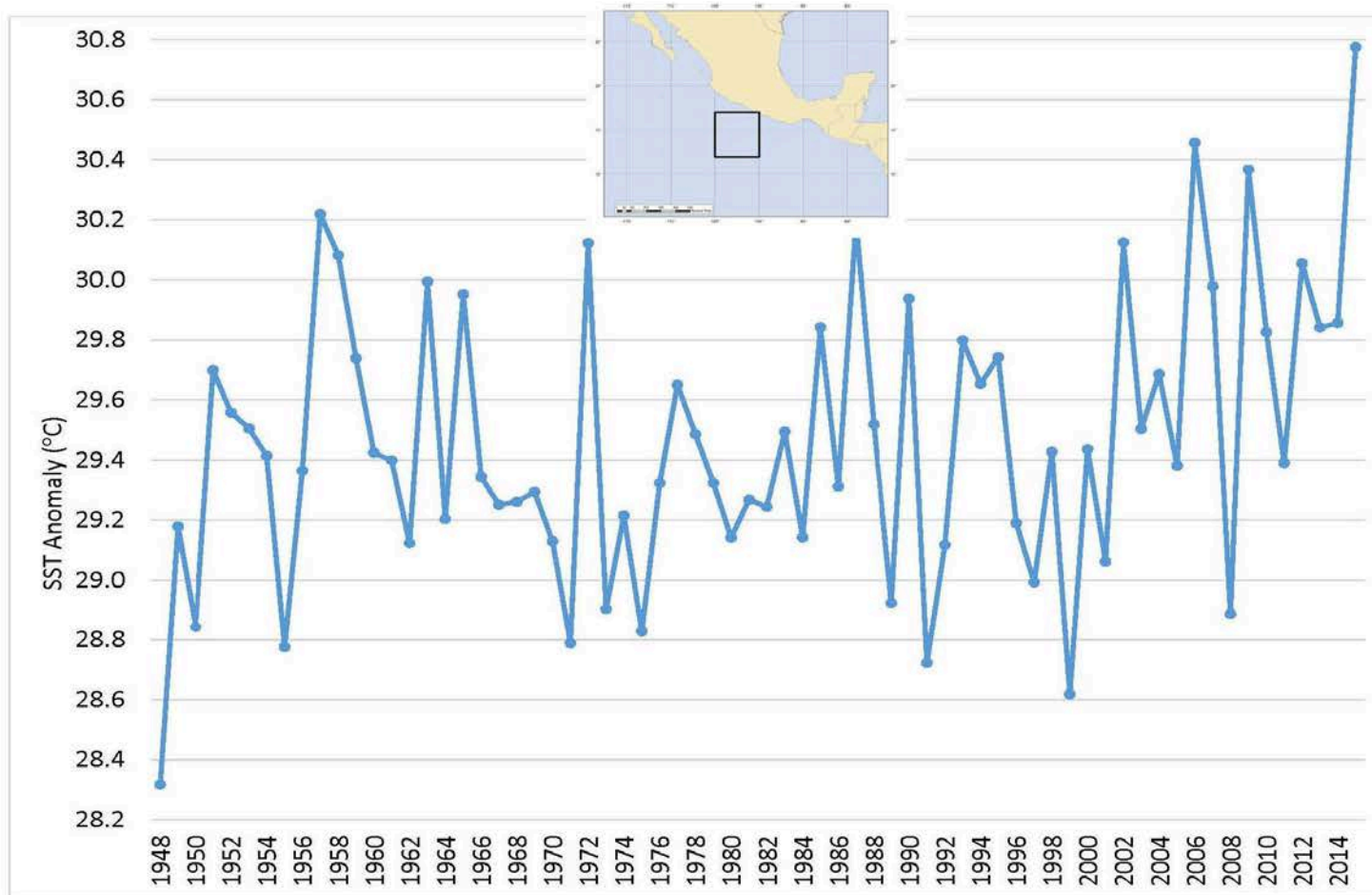
Figure 7. Sea surface temperatures from 13°-17°N and 100°-105°W averaged over a 10-day period prior to the passage of Patricia. Source NCEP/NCAR Reanalysis data base.
