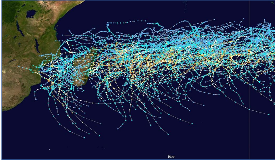
Figure 26: Southwest Indian Ocean tropical cyclone tracks from 1980-2005.
