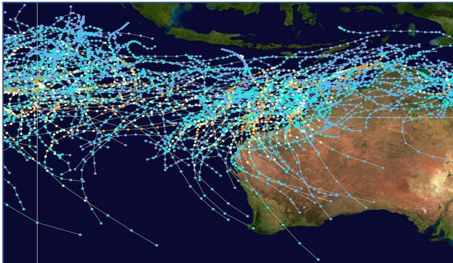
Figure 27: Southeast Indian Ocean tropical cyclone tracks from 1980-2005.
