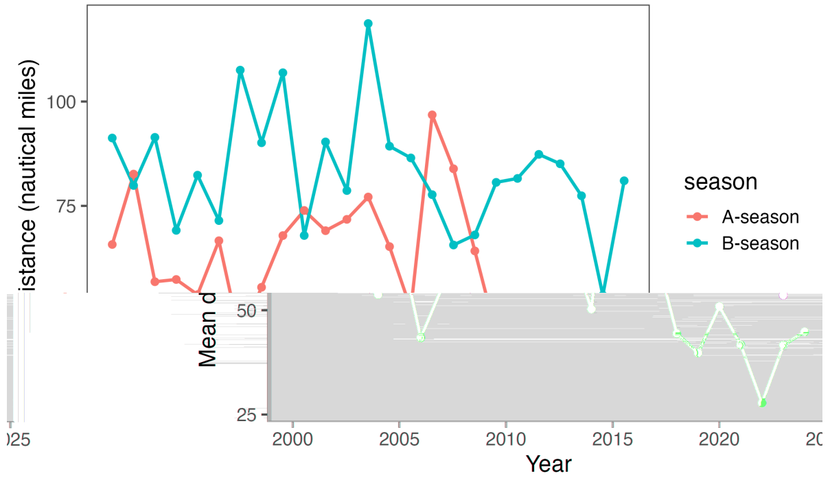
Figure 8: Estimated mean daily distance between operations, 2000-2024.
