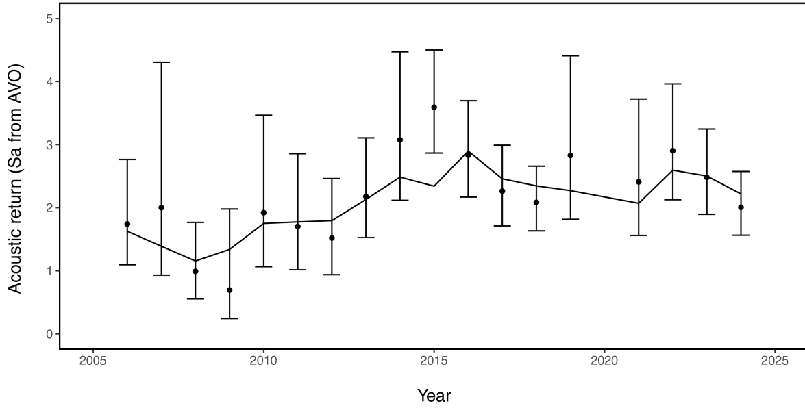
Figure 44: Model results of predicted and observed AVO index. Error bars represent assumed 95% confidence bounds of the input series.
