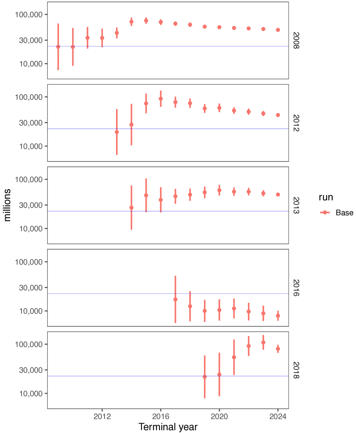
Figure 56: Retrospective evolution of EBS pollock selected year-class estimates as a function of the terminal year of data used in the model (based on retrospectives of Model 23.0).
