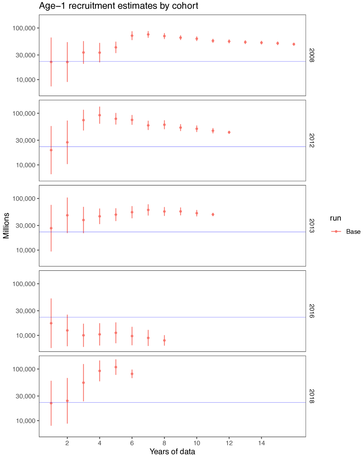
Figure 57: Retrospective evolution of EBS pollock selected year-class estimates as a function of the the number of years the year-class has been in the model (based on retrospectives of Model 23.0).
