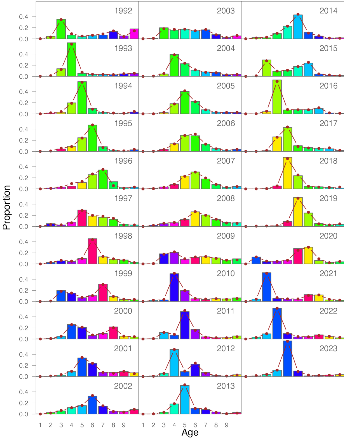
Figure 35: Model fit (dots) to the EBS pollock fishery proportion-at-age data (columns; 1992–2023). The 2023 data are new to this year’s assessment. Colors coincide with cohorts progressing through time.
