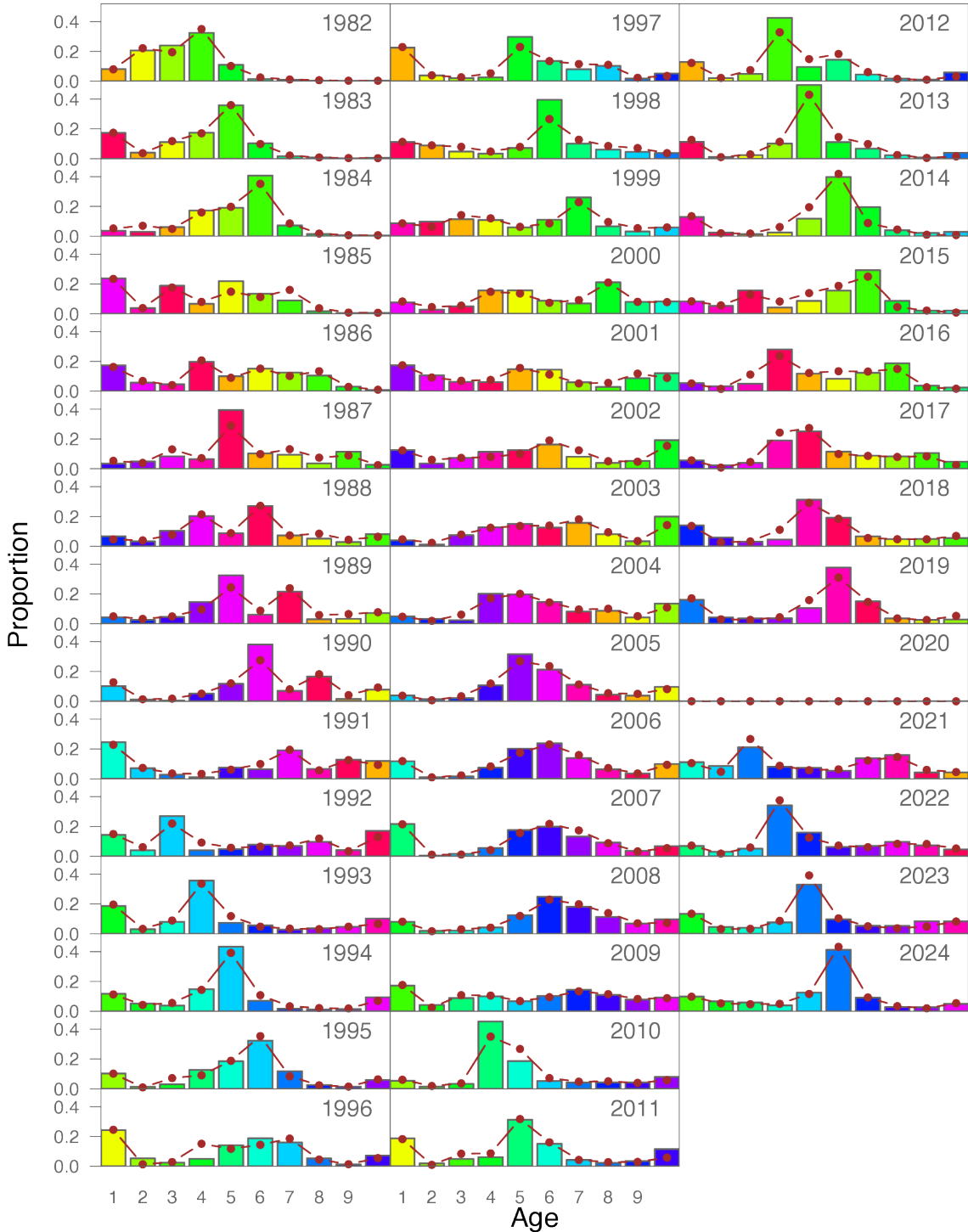
Figure 37: Model fit (dots) to the bottom trawl survey proportion-at-age composition data (columns) for EBS pollock. Colors correspond to cohorts over time.
