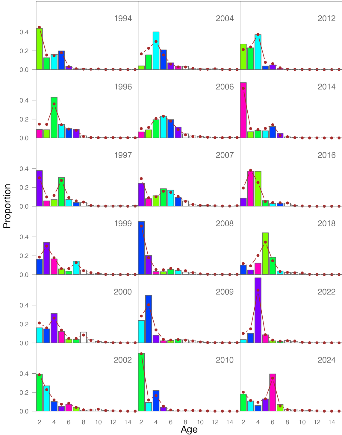
Figure 39: Model fit (dots) to the acoustic-trawl survey proportion-at-age composition data (columns) for EBS pollock. Colors correspond to cohorts over time (for years with consecutive surveys).
