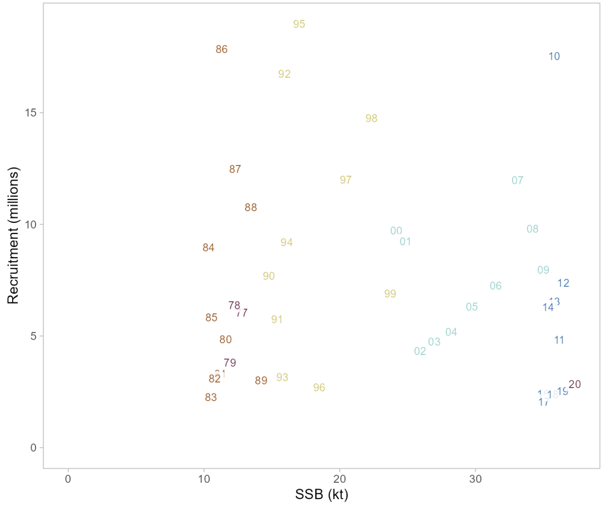
Figure 12-8. Scatterplot of spawner-recruit estimates for the GOA dusky rockfish author's recommended model.
