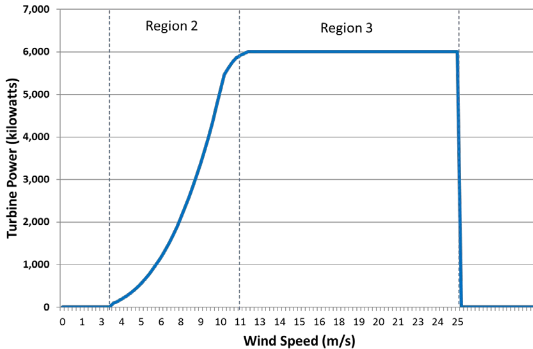
Figure 9. Generic 6-MW power curve for representative wind turbine technology available for commercial deployment in 2015 (assumed operation date of 2017)
