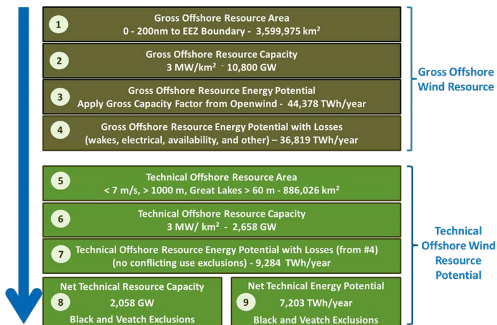
Figure 2. Progression of analysis for the 2016 Offshore Wind Energy Resource Assessment for the United States
