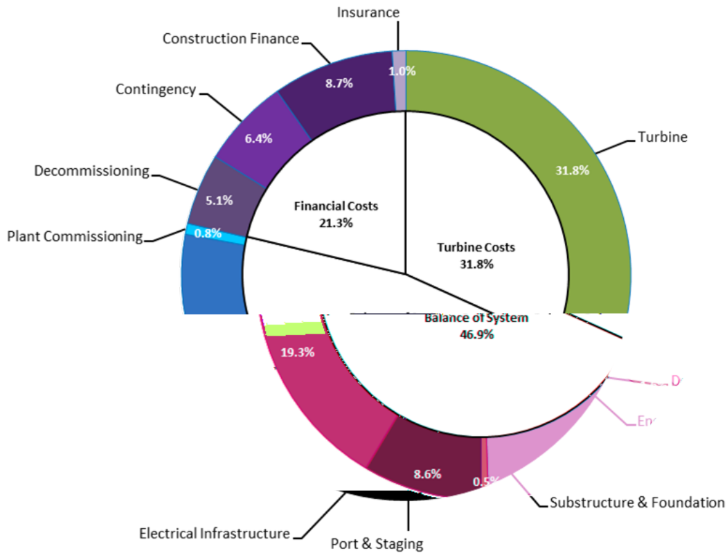
Figure 14. Capital expenditures for the 2015 fixed-bottom offshore wind reference project Source: NREL
