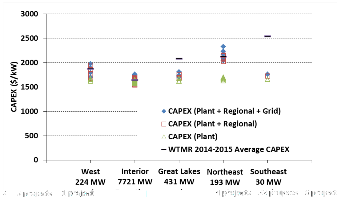
Figure 10. CapEx estimated for locations where projects were installed in 2015 including the wind plant, regional cost increment, and grid connection cost increment (wind technologies market report [WTMR])
