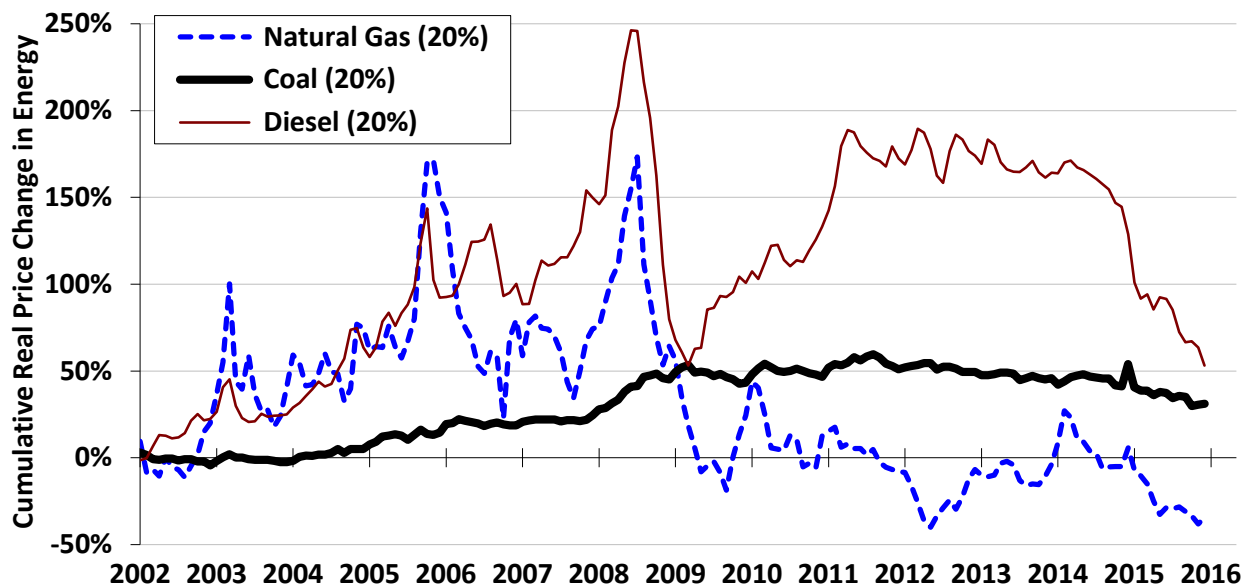
Figure 31. Cumulative change in energy input costs
