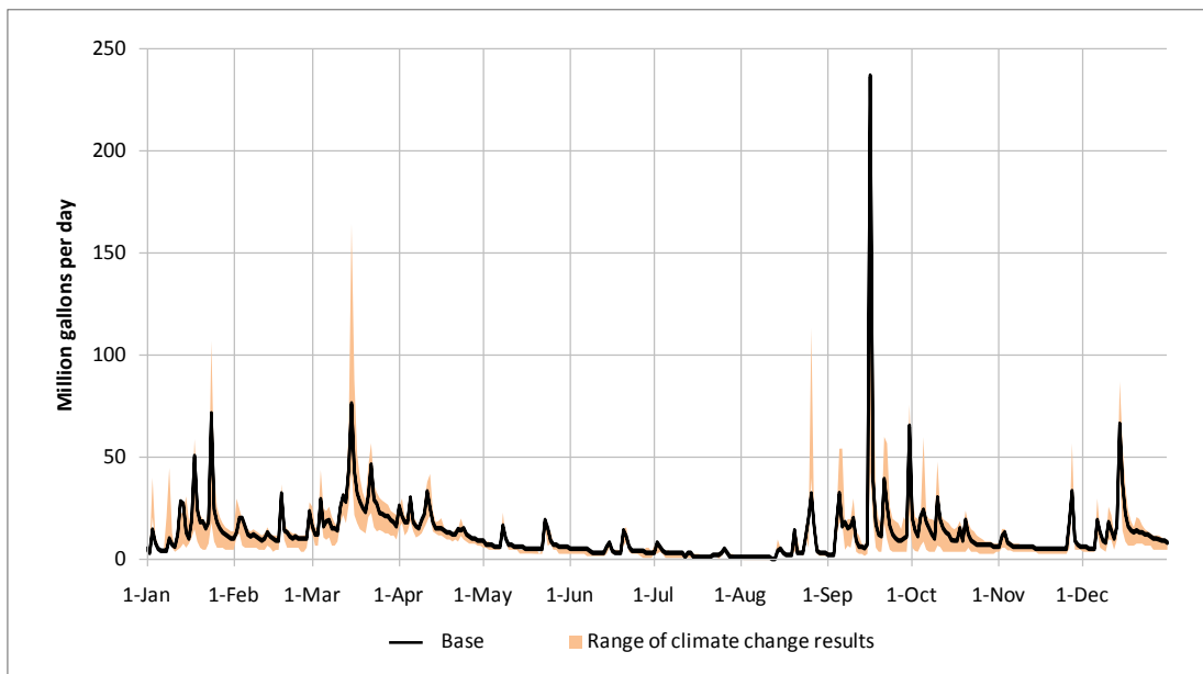
Figure 6-8: Little Seneca Reservoir inflow in the year 2040 in the event of a moderate drought.
