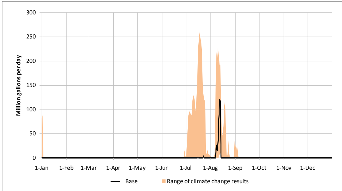
Figure 6-17: Little Seneca releases in the year 2040 in the event of a moderate drought.
