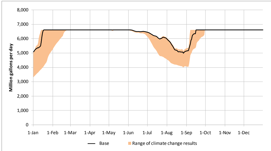
Figure 6-13: Occoquan Reservoir storage in the year 2040 in the event of a moderate drought.
