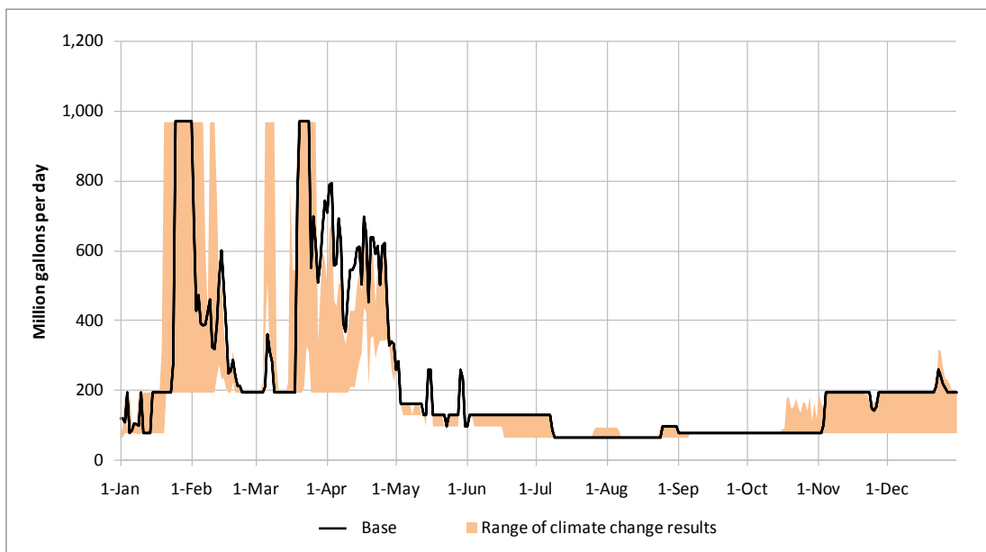
Figure 6-16: Jennings Randolph water quality releases in the year 2040 in the event of a moderate drought.
