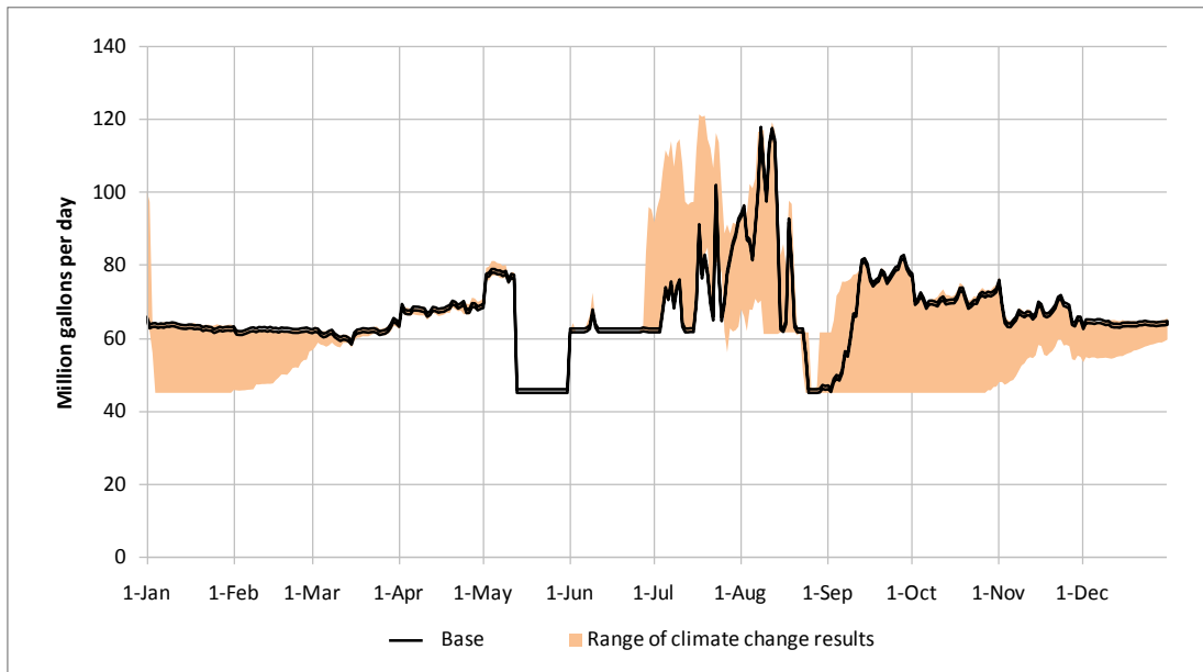
Figure 6-18: Occoquan production in the year 2040 in the event of a moderate drought.
