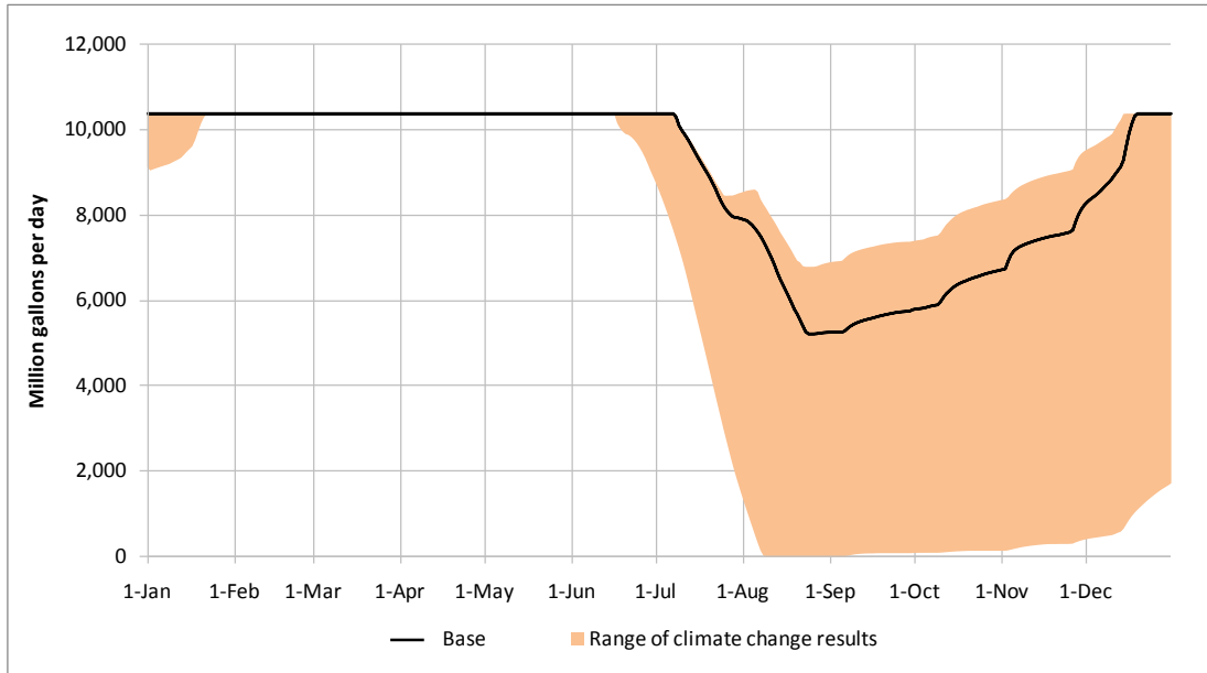
Figure 6-9: Jennings Randolph Reservoir water supply storage in the year 2040 in the event of a moderate drought.
