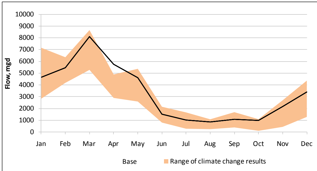
Figure 5-6: Savage Reservoir total monthly inflows averaged over the 12-year simulation period.
