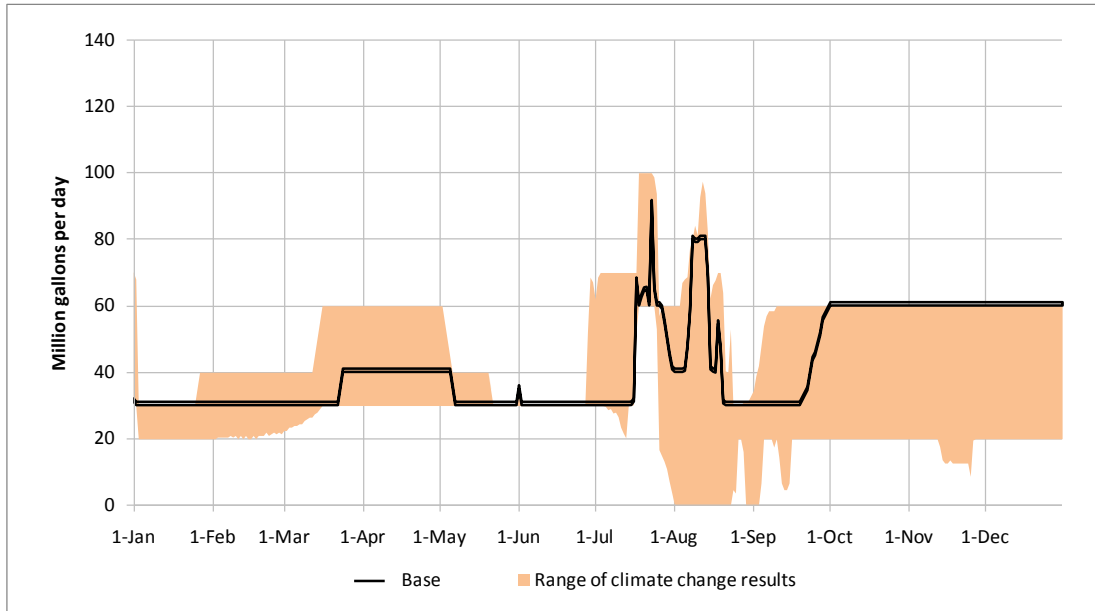
Figure 6-19: Patuxent production in the year 2040 in the event of a moderate drought.
