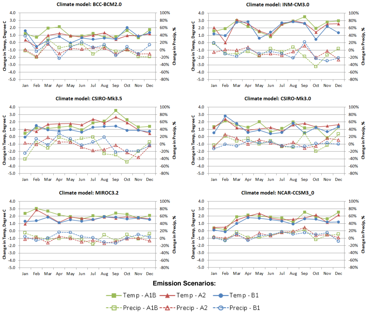
Figure 5-1: Change in basinwide monthly average air temperature (°C) and monthly total precipitation (%) for different climate models and emission scenarios.
