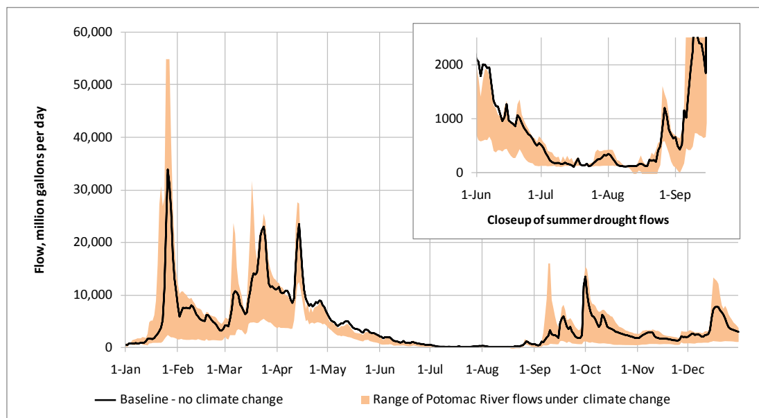
Figure ES-2: Projected Potomac River flow at Little Falls dam during a moderate drought in the year 2040, assuming no changes to the current water supply system.
