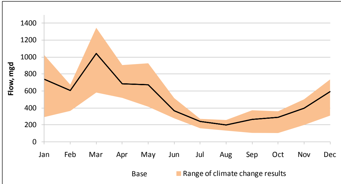
Figure 5-7: Little Seneca Reservoir total monthly inflows averaged over the 12-year simulation period.
