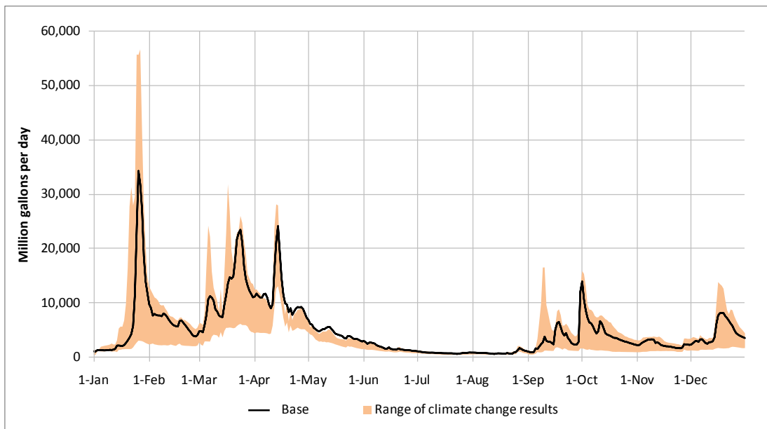
Figure 6-2: “Natural” Potomac River flow at Little Falls in the year 2040 in the event of a moderate drought.
