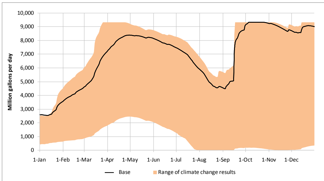
Figure 6-12: Combined Patuxent reservoirs (Tridelphia and Rocky Gorge) storage in the year 2040 in the event of a moderate drought.
