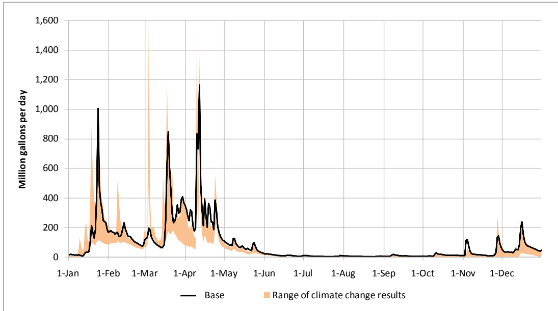
Figure 6-5: Savage Reservoir inflow in the year 2040 in the event of a moderate drought.
