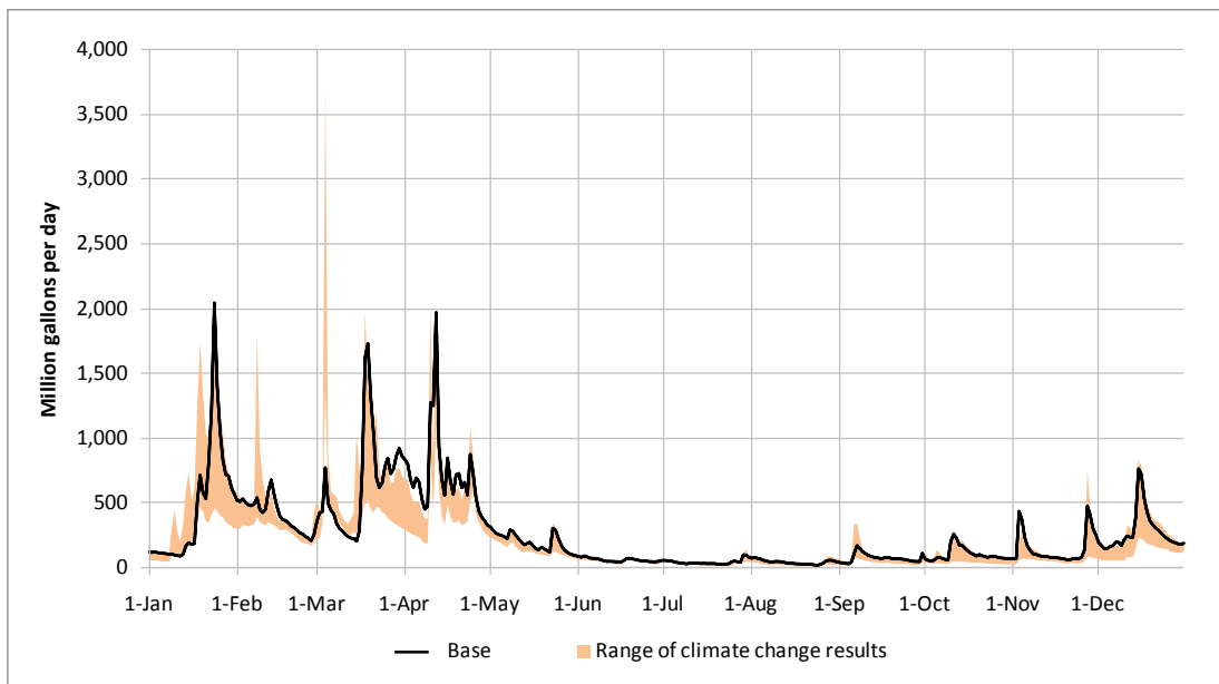
Figure 6-4: Jennings Randolph Reservoir inflow in the year 2040 in the event of a moderate drought.
