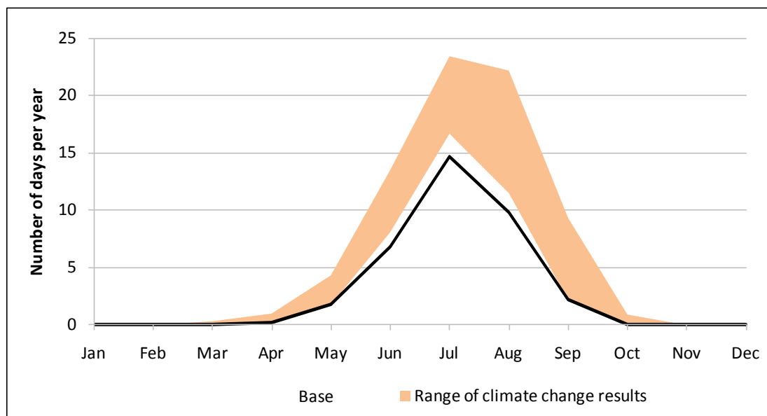
Figure 5-2: Average number of days per year with maximum temperatures above 32.2°C (90°F). Data is for land segment A11001 (which includes Washington Reagan Airport, NCDC Station ID 448906).
