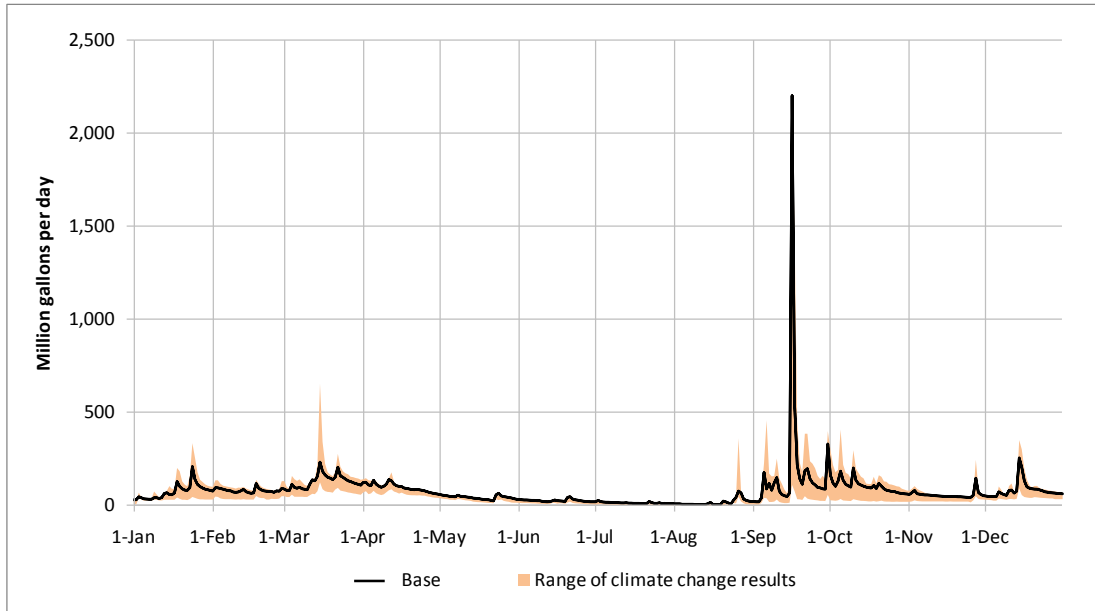
Figure 6-7: Patuxent reservoirs inflow in the year 2040 in the event of a moderate drought.
