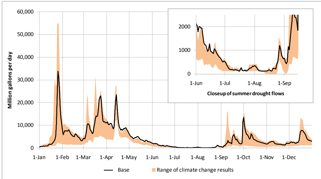
Figure 6-3: Potomac River flow at Little Falls in the year 2040 in the event of a moderate drought.
