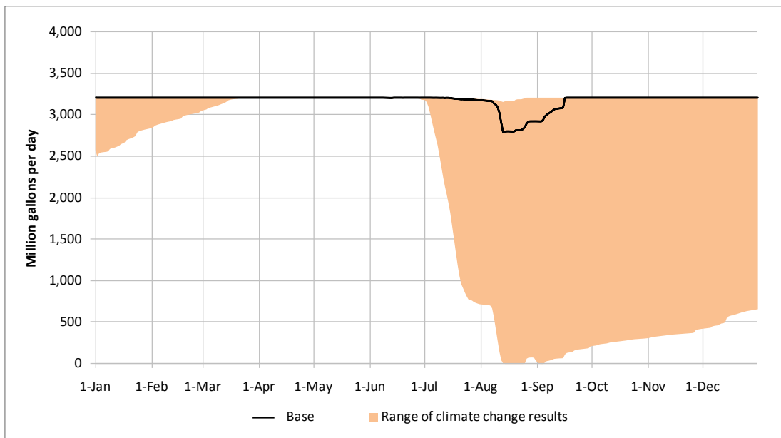
Figure 6-14: Little Seneca storage in the year 2040 in the event of a moderate drought.
