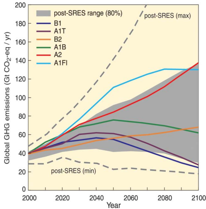
Figure 3-1: Projections of global greenhouse gas (GHG) emissions, under a variety of hypothetical emissions scenarios (B1, A1T, B2, A1B, A2, and A1FI), for the next century in the absence of additional climate policies, expressed in gigatons of carbon dioxide equivalent emissions per year (reprinted from IPCC, 2007c).
