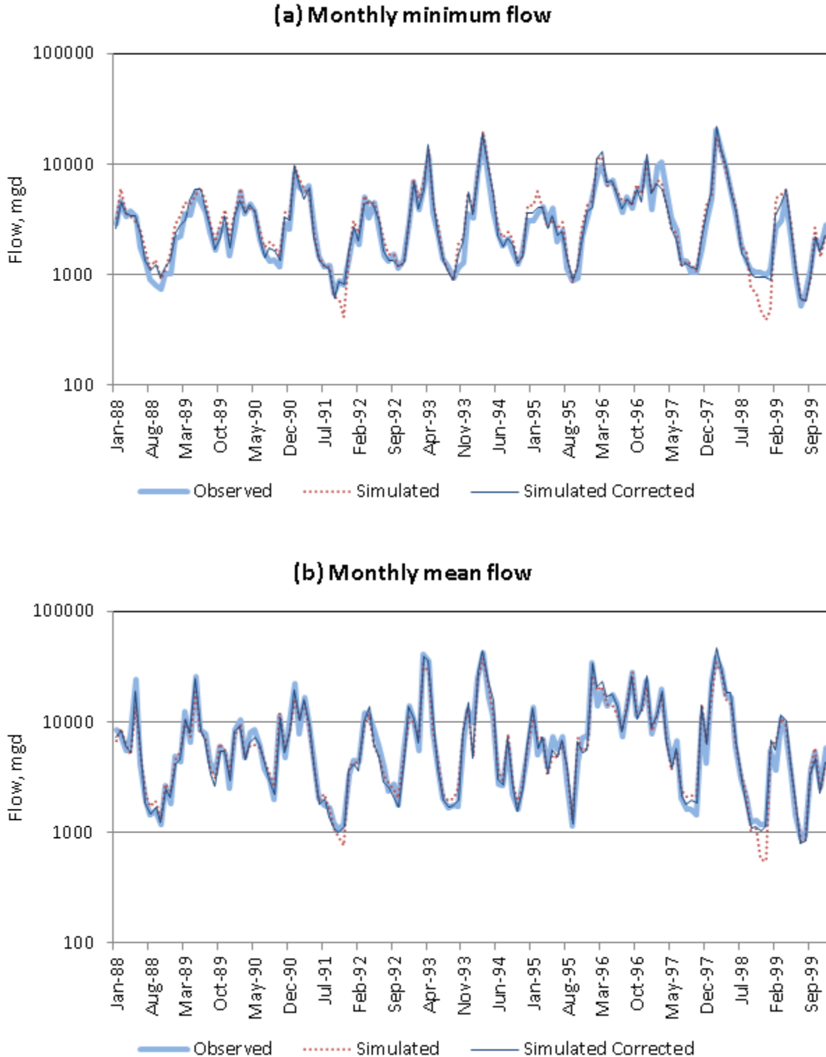
Figure 4-3: Observed, (uncorrected) simulated, and bias-corrected simulated Potomac River flow at Little Falls (with effects of WMA withdrawals, contributions from JR, S, and LS reservoir watersheds, and estimated upstream consumptive use removed).
