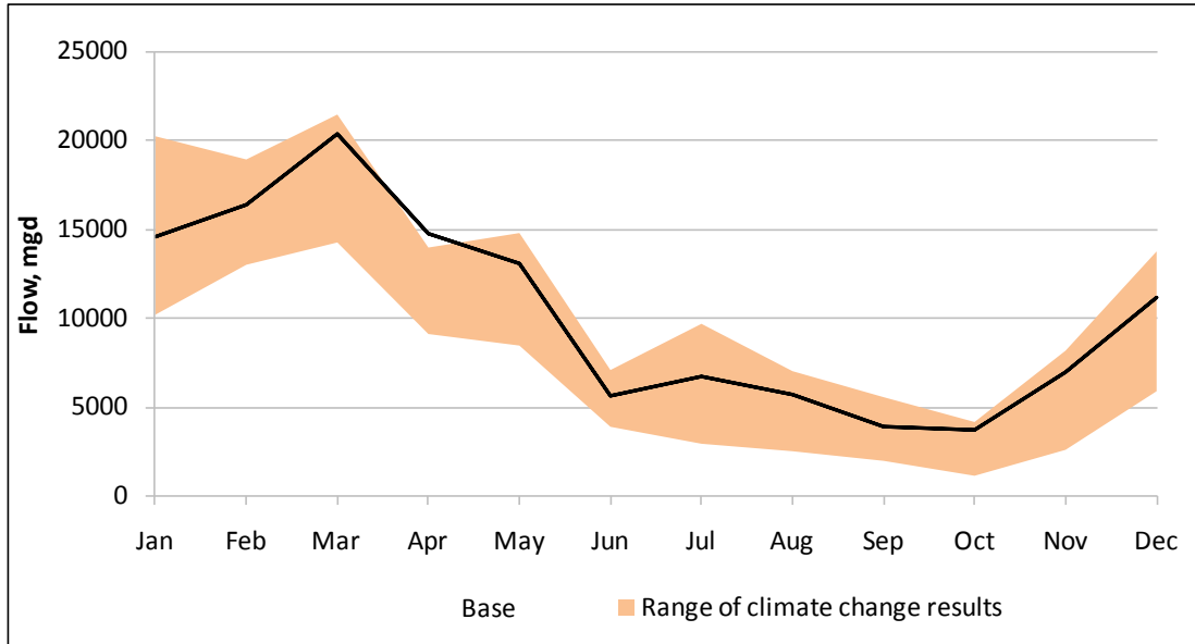
Figure 5-5: Jennings Randolph Reservoir total monthly inflows averaged over the 12-year simulation period.
