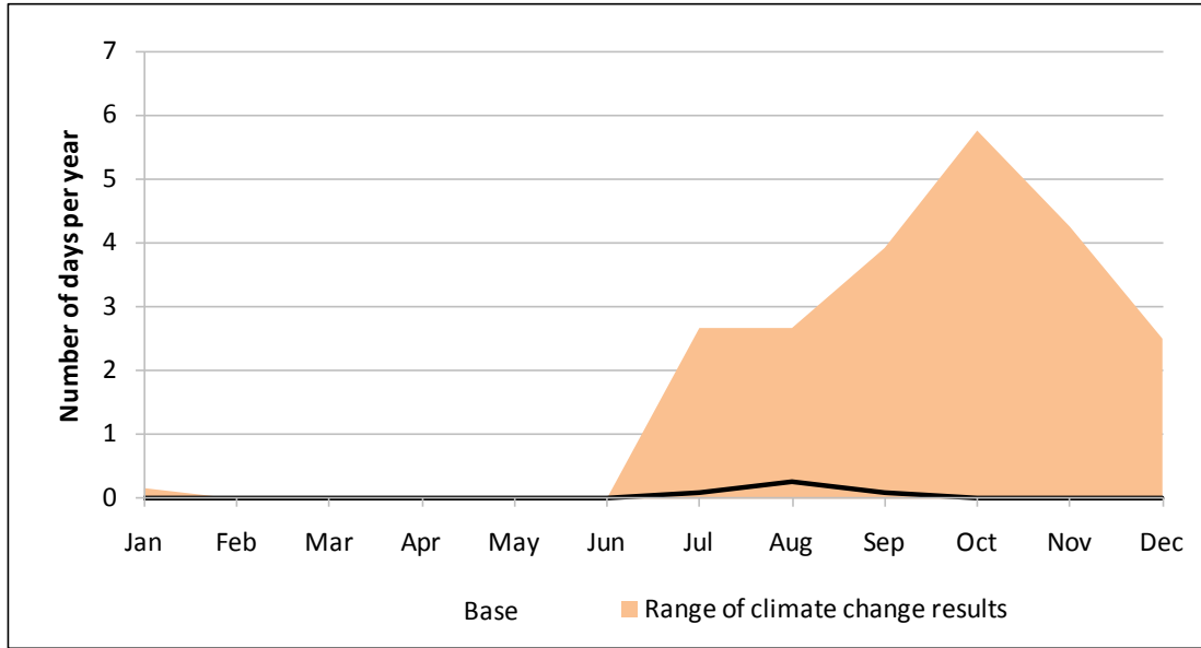
Figure 5-3: Average number of days per year that natural Potomac River flow at Little Falls fell below 700 mgd.
