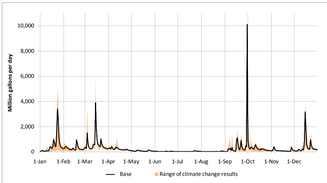
Figure 6-6: Occoquan Reservoir inflow in the year 2040 in the event of a moderate drought.
