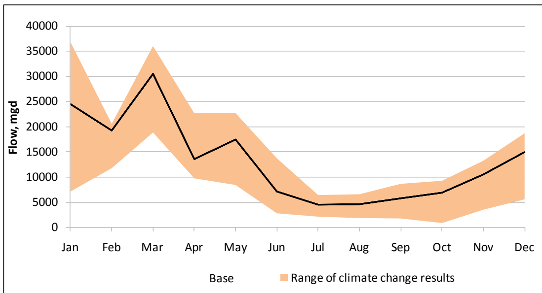
Figure 5-8: Ocoquan Reservoir total monthly inflows averaged over the 12-year simulation period.
