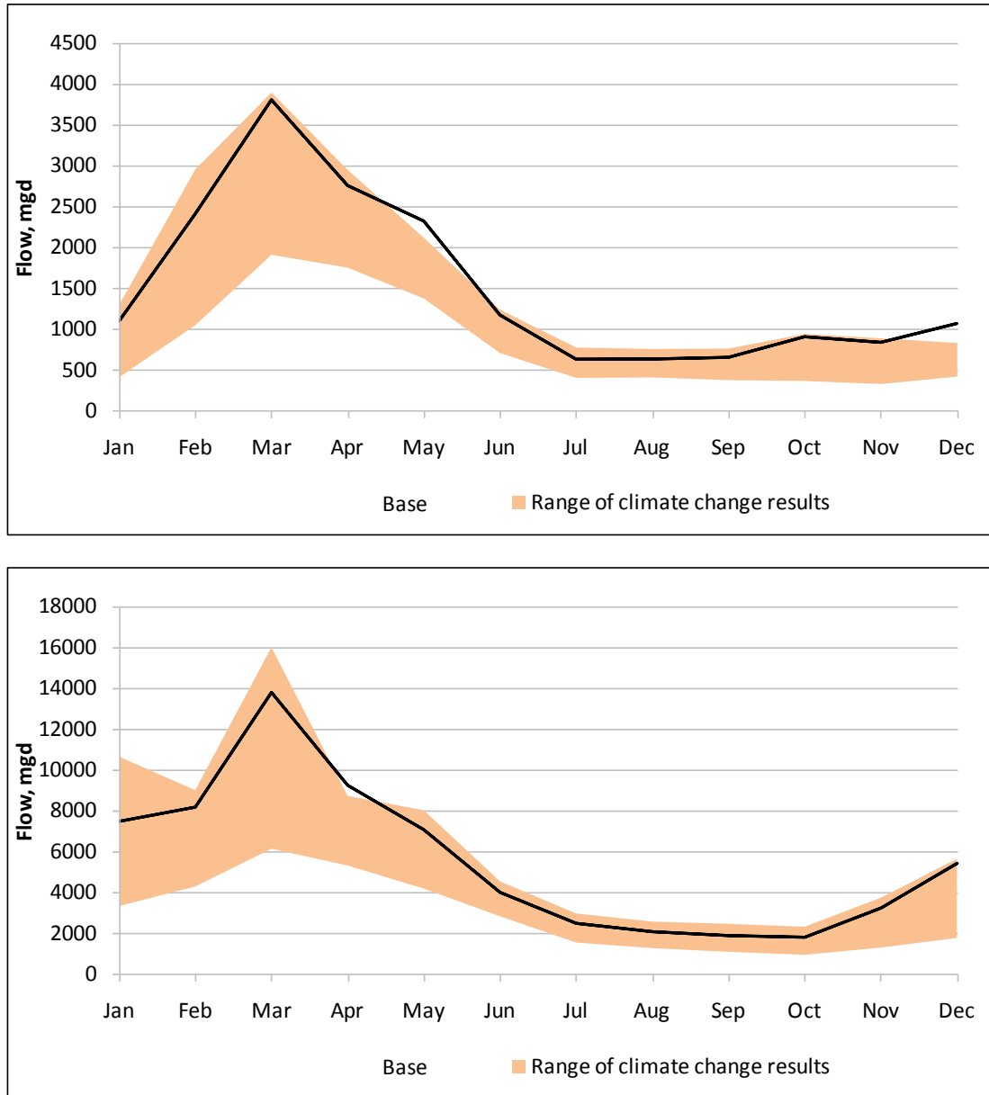
Figure 5-4: Monthly minimum (top graph) and median (bottom graph) natural Potomac River flow at Little Falls.
