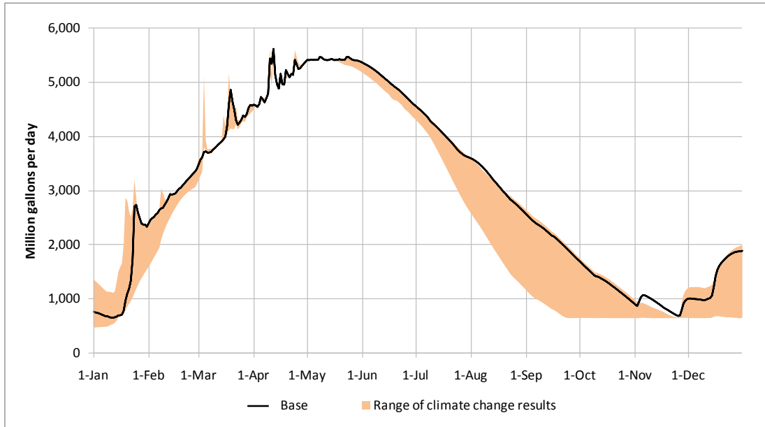
Figure 6-11: Savage Reservoir storage in the year 2040 in the event of a moderate drought.
