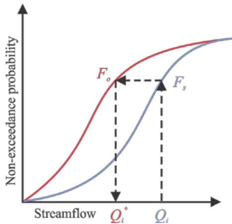
Figure 4-2: Quantile mapping concept, where F_s is the cumulative probability distribution for simulated stream flow, F_o is the cumulative probability distribution for observed stream flow, Q_i is the simulated stream flow, and Q_i^* is the simulated stream flow after being adjusted (image modified from Kim, 2009).
