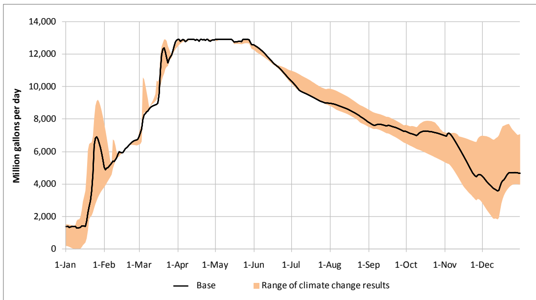
Figure 6-10: Jennings Randolph Reservoir water quality storage in the year 2040 in the event of a moderate drought.
