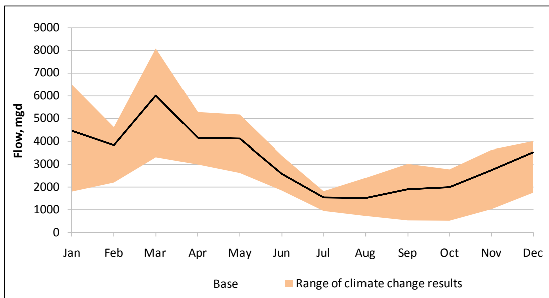
Figure 5-9: Patuxent reservoirs (Tridelphia and Rocky Gorge) total monthly inflows averaged over the 12-year simulation period.
