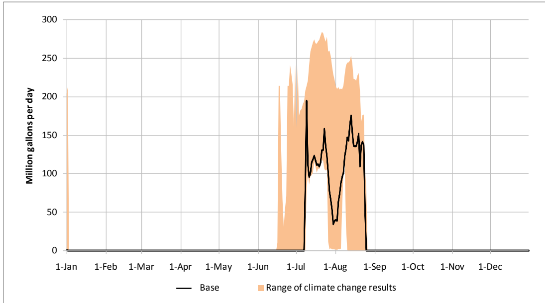
Figure 6-15: Jennings water supply releases in the year 2040 in the event of a moderate drought.
