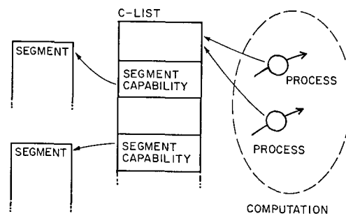
FIG. 1. A computation
