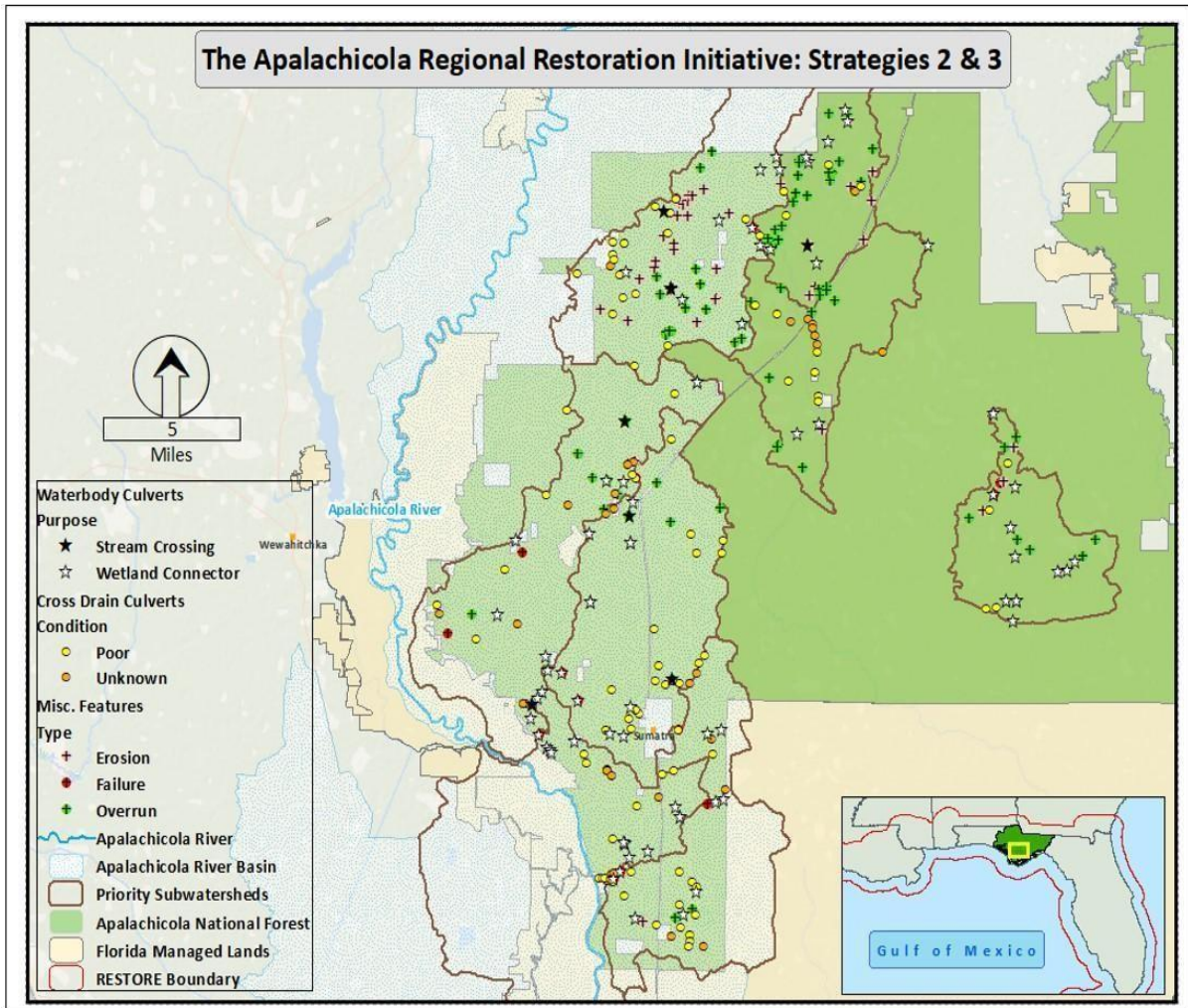
Figure 5: Priority hydrological infrastructure on the Apalachicola National Forest (ANF) for installation, repair, replacement, or modification. Selection was based on five factors: 1) number of high priority waterbody culvert replacements, 2) number of cross drains in poor or unknown condition, 3) number of erosion events, significant failures, or overrun road points, 4) drainage bay, 5) percent of sub watershed on the ANF (all hydrologic assessment field data collected through Tate’s Hell Strategy 1 project).
