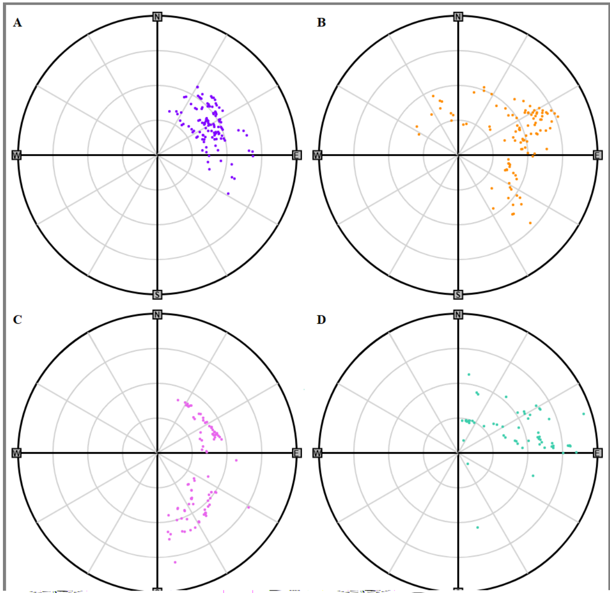
Figure 8: As in Fig. 6, but color-coded by TC for the top four TCTOR-era systems from Table 1: a) Ivan (2004, purple), b) Frances (2004, yellow-orange), c) Rita (2005, pink), and d) Katrina (2005, green-blue).
