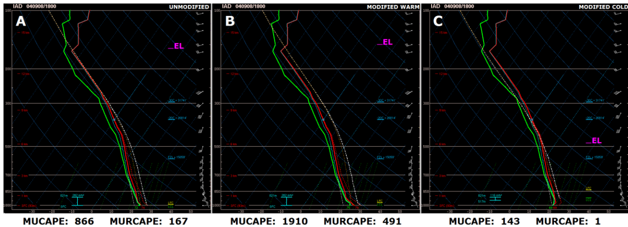
Figure 1: Skew T - \log p diagrams of the Dulles, VA (IAD) sounding, 1800 UTC 8 September 2004—in proximity (as defined in the text) to four tornadoes produced by Tropical Depression Frances. Sounding is: a) unmodified, as observed; b) with surface temperature and dewpoint increased 5°F (2.7°C) and 3°F (1.7°C) respectively, using a thermally dry-adiabatic, constant-mixing-ratio assumption for the mixed layer; c) with surface temperature and dewpoint likewise cooled 5°F (2.7°C) and 3°F (1.7°C) respectively. Most-unstable (MU) parcel CAPE and RCAPE ( \text{J kg}^{-1} ) values shown beneath each diagram. Parcel trace (dotted white line) and virtual temperature correction (dotted red line) shown for MUCAPE. Equilibrium level (EL), same as LNB, is highlighted in magenta. Cyan bar represents effective inflow layer (Thompson et al. 2007), which is surface-based for (a) and (b). Click image to enlarge.
